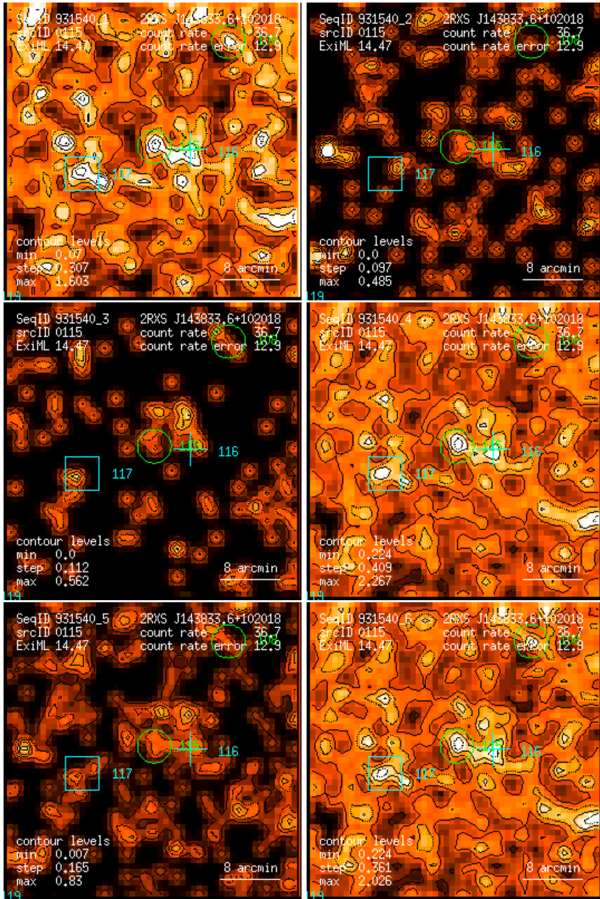
Figure 115: RASS 931540: detection 0115: band rate images, Gaussian filter: (1) PSPC channels 11 – 41, (2) 52 – 90, (3) 91 – 201, (4) 11 – 235, (5) 52 – 201, (6) 11 – 201. Broad band rates in counts/ks. Band rate contour levels in counts/ks/arcmin 2 .
