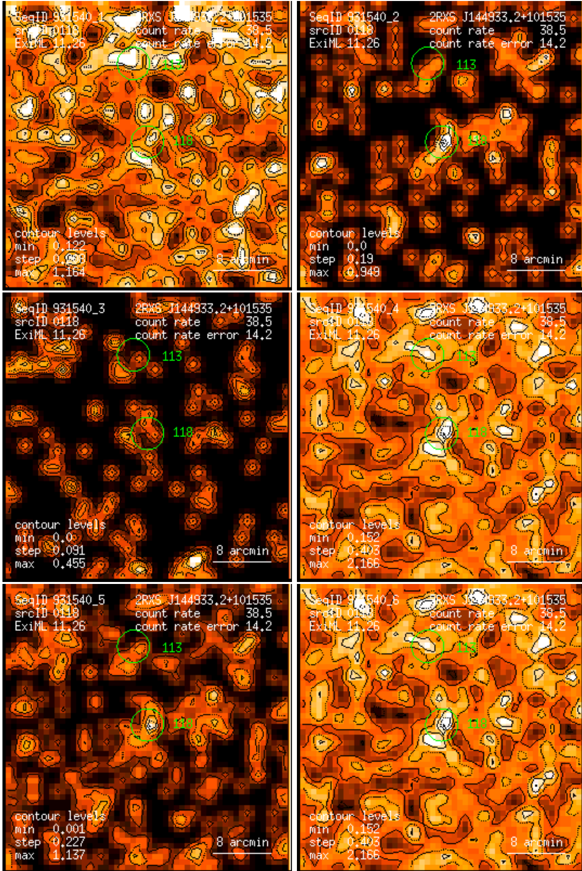
Figure 118: RASS 931540: detection 0118: band rate images, Gaussian filter: (1) PSPC channels 11 – 41, (2) 52 – 90, (3) 91 – 201, (4) 11 – 235, (5) 52 – 201, (6) 11 – 201. Broad band rates in counts/ks. Band rate contour levels in counts/ks/arcmin 2 .
