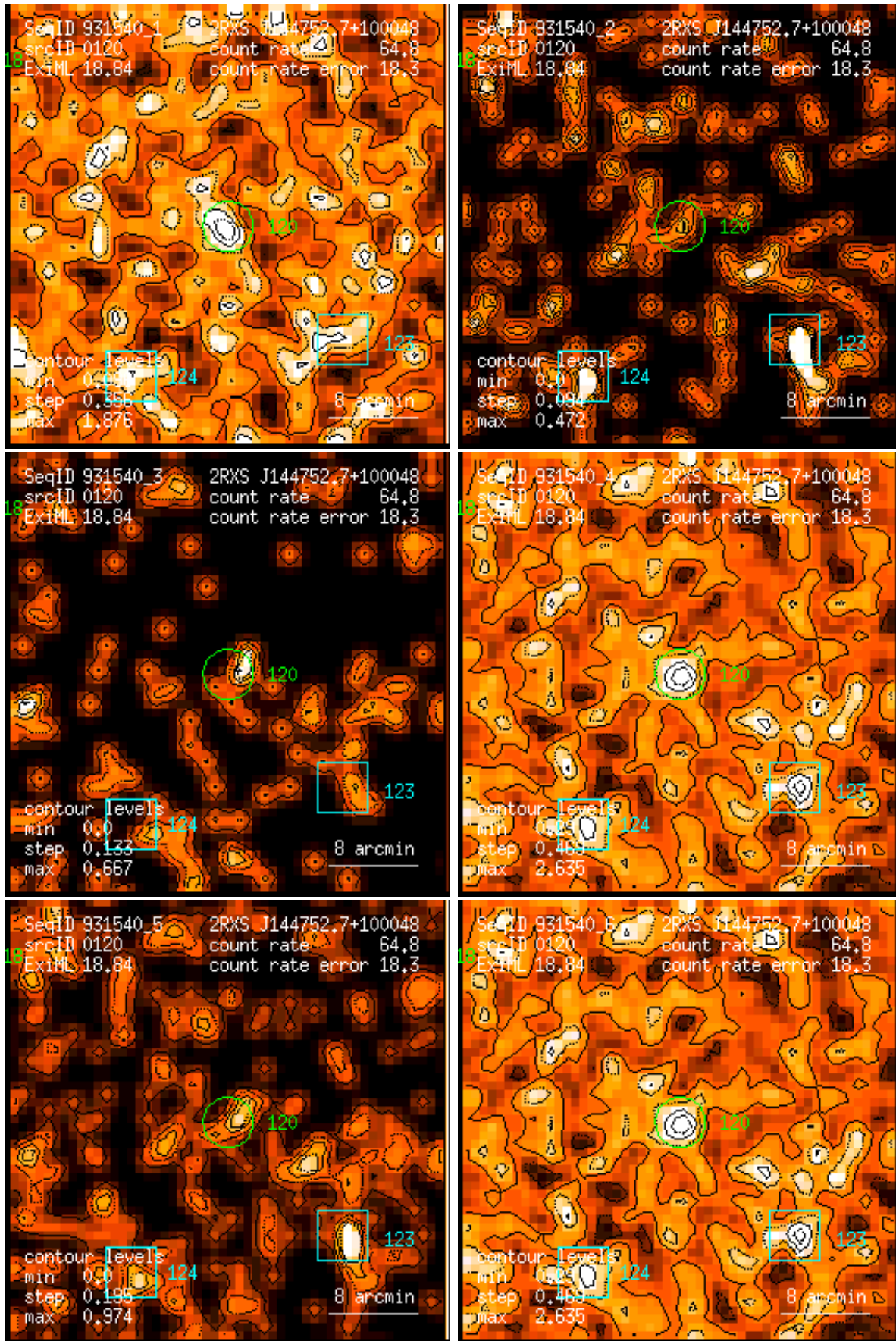
Figure 120: RASS 931540: detection 0120: band rate images, Gaussian filter: (1) PSPC channels 11 – 41, (2) 52 – 90, (3) 91 – 201, (4) 11 – 235, (5) 52 – 201, (6) 11 – 201. Broad band rates in counts/ks. Band rate contour levels in counts/ks/arcmin 2 .
