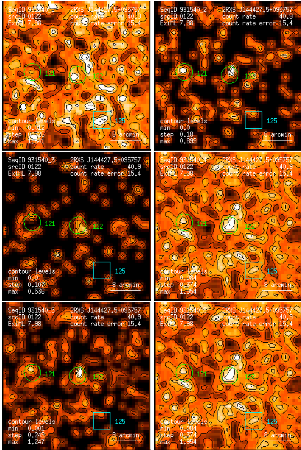
Figure 122: RASS 931540: detection 0122: band rate images, Gaussian filter: (1) PSPC channels 11 – 41, (2) 52 – 90, (3) 91 – 201, (4) 11 – 235, (5) 52 – 201, (6) 11 – 201. Broad band rates in counts/ks. Band rate contour levels in counts/ks/arcmin 2 .
