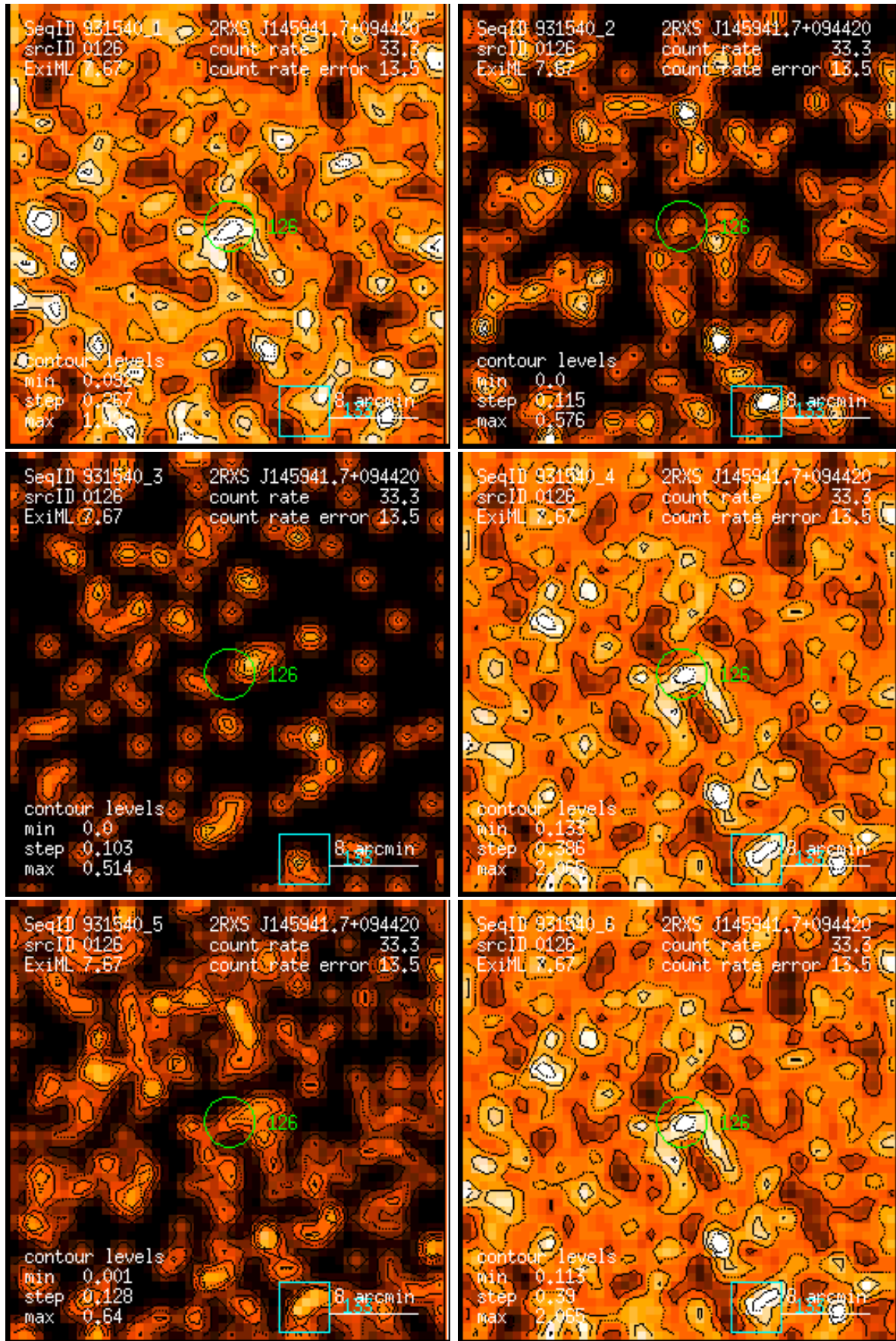
Figure 126: RASS 931540: detection 0126: band rate images, Gaussian filter: (1) PSPC channels 11 – 41, (2) 52 – 90, (3) 91 – 201, (4) 11 – 235, (5) 52 – 201, (6) 11 – 201. Broad band rates in counts/ks. Band rate contour levels in counts/ks/arcmin 2 .
