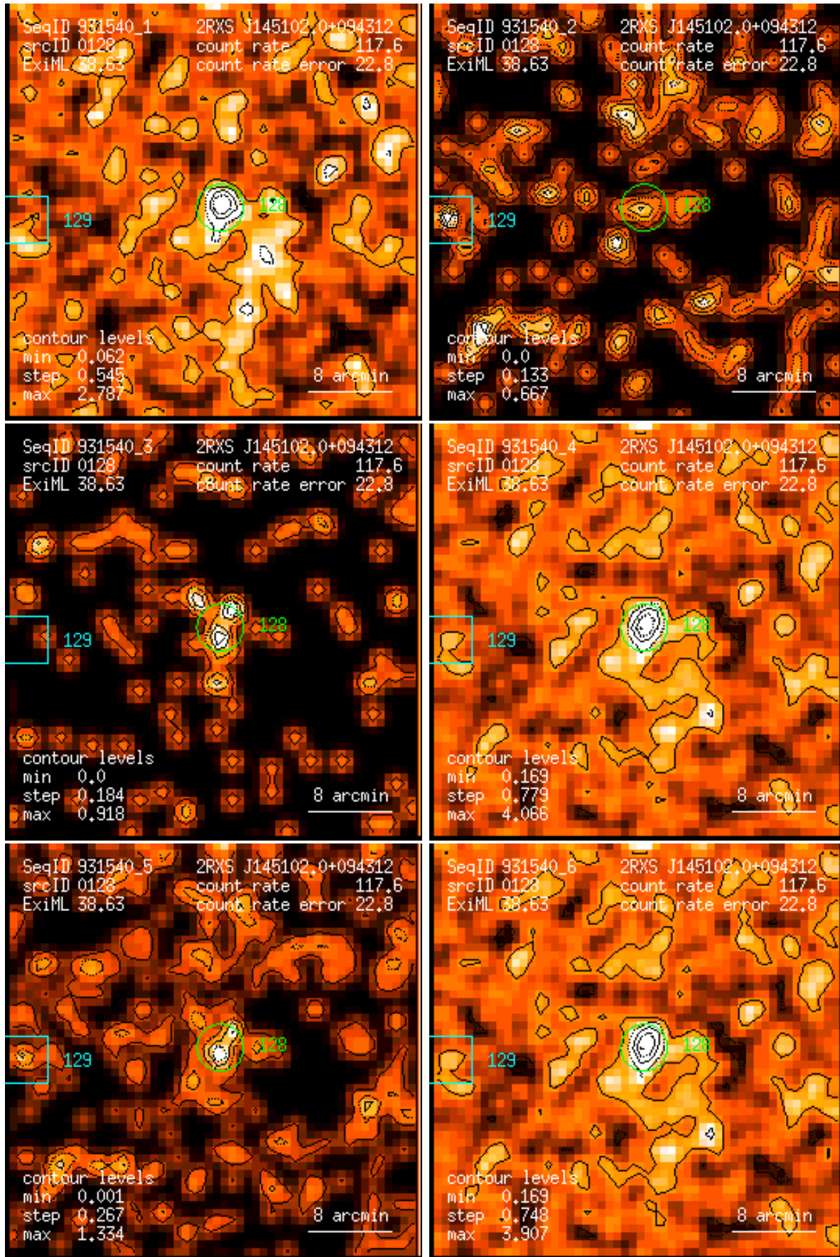
Figure 128: RASS 931540: detection 0128: band rate images, Gaussian filter: (1) PSPC channels 11 – 41, (2) 52 – 90, (3) 91 – 201, (4) 11 – 235, (5) 52 – 201, (6) 11 – 201. Broad band rates in counts/ks. Band rate contour levels in counts/ks/arcmin 2 .
