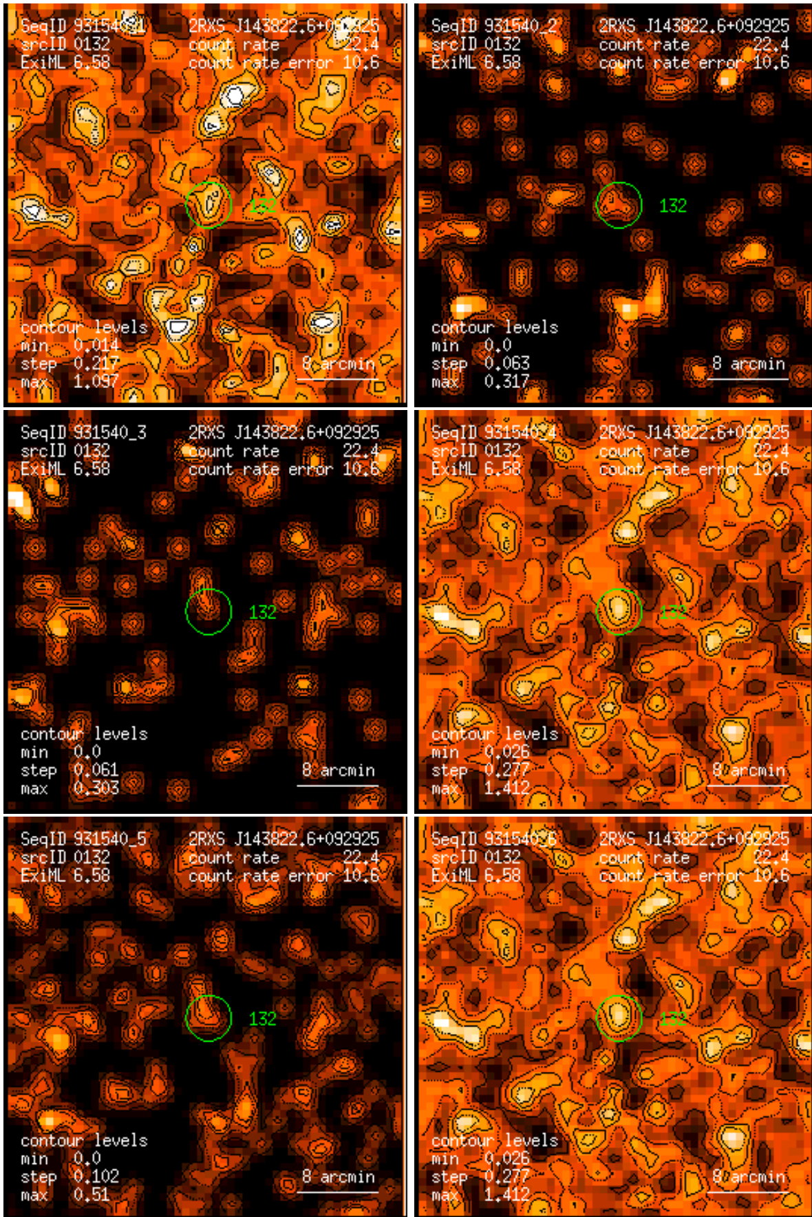
Figure 132: RASS 931540: detection 0132: band rate images, Gaussian filter: (1) PSPC channels 11 – 41, (2) 52 – 90, (3) 91 – 201, (4) 11 – 235, (5) 52 – 201, (6) 11 – 201. Broad band rates in counts/ks. Band rate contour levels in counts/ks/arcmin 2 .
