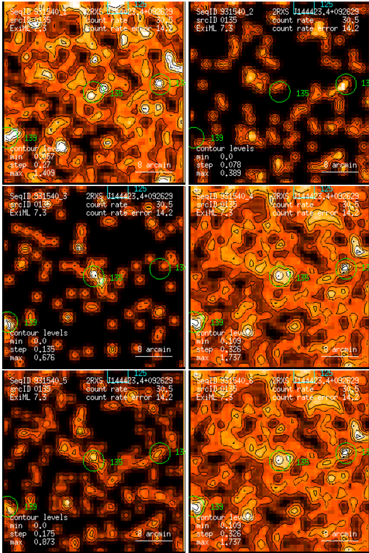
Figure 135: RASS 931540: detection 0135: band rate images, Gaussian filter: (1) PSPC channels 11 – 41, (2) 52 – 90, (3) 91 – 201, (4) 11 – 235, (5) 52 – 201, (6) 11 – 201. Broad band rates in counts/ks. Band rate contour levels in counts/ks/arcmin 2 .
