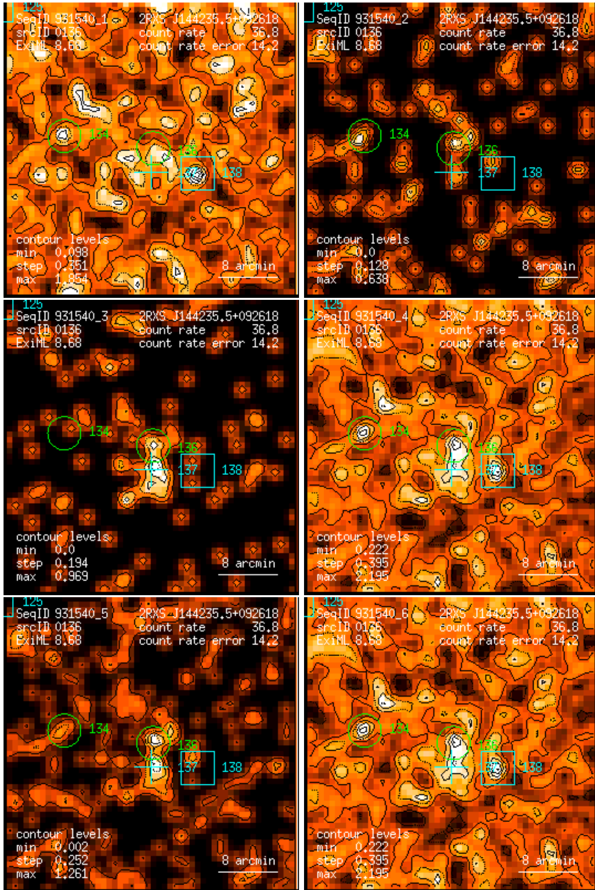
Figure 136: RASS 931540: detection 0136: band rate images, Gaussian filter: (1) PSPC channels 11 – 41, (2) 52 – 90, (3) 91 – 201, (4) 11 – 235, (5) 52 – 201, (6) 11 – 201. Broad band rates in counts/ks. Band rate contour levels in counts/ks/arcmin 2 .
