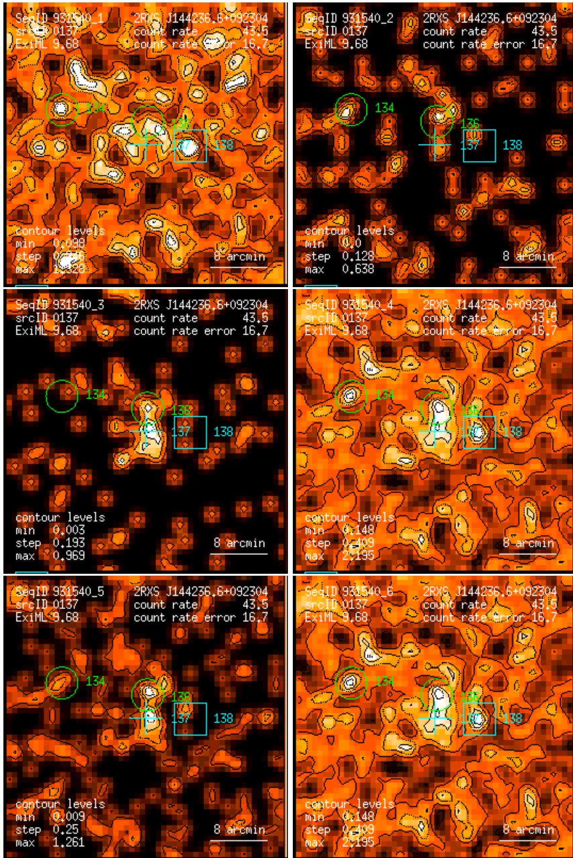
Figure 137: RASS 931540: detection 0137: band rate images, Gaussian filter: (1) PSPC channels 11 – 41, (2) 52 – 90, (3) 91 – 201, (4) 11 – 235, (5) 52 – 201, (6) 11 – 201. Broad band rates in counts/ks. Band rate contour levels in counts/ks/arcmin 2 .
