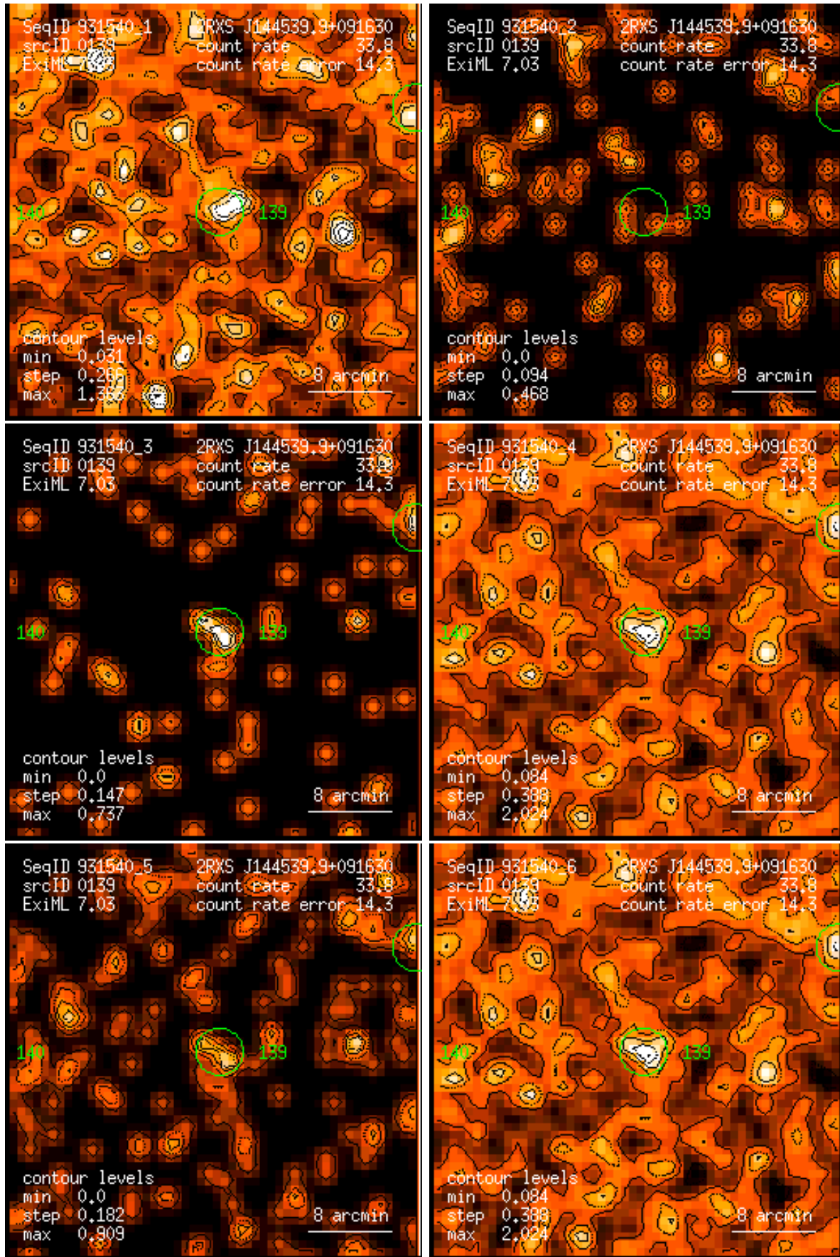
Figure 139: RASS 931540: detection 0139: band rate images, Gaussian filter: (1) PSPC channels 11 – 41, (2) 52 – 90, (3) 91 – 201, (4) 11 – 235, (5) 52 – 201, (6) 11 – 201. Broad band rates in counts/ks. Band rate contour levels in counts/ks/arcmin 2 .
