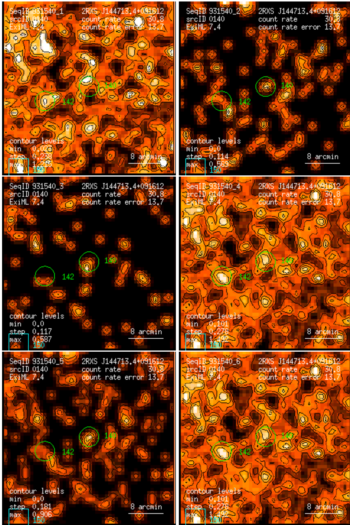
Figure 140: RASS 931540: detection 0140: band rate images, Gaussian filter: (1) PSPC channels 11 – 41, (2) 52 – 90, (3) 91 – 201, (4) 11 – 235, (5) 52 – 201, (6) 11 – 201. Broad band rates in counts/ks. Band rate contour levels in counts/ks/arcmin 2 .
