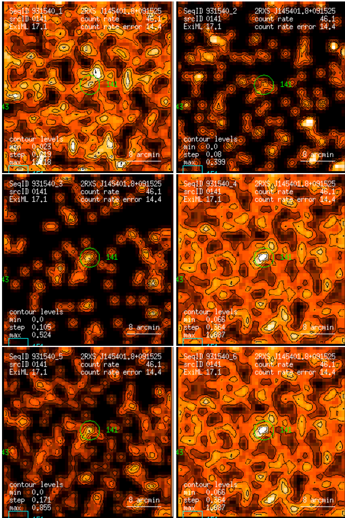
Figure 141: RASS 931540: detection 0141: band rate images, Gaussian filter: (1) PSPC channels 11 – 41, (2) 52 – 90, (3) 91 – 201, (4) 11 – 235, (5) 52 – 201, (6) 11 – 201. Broad band rates in counts/ks. Band rate contour levels in counts/ks/arcmin 2 .
