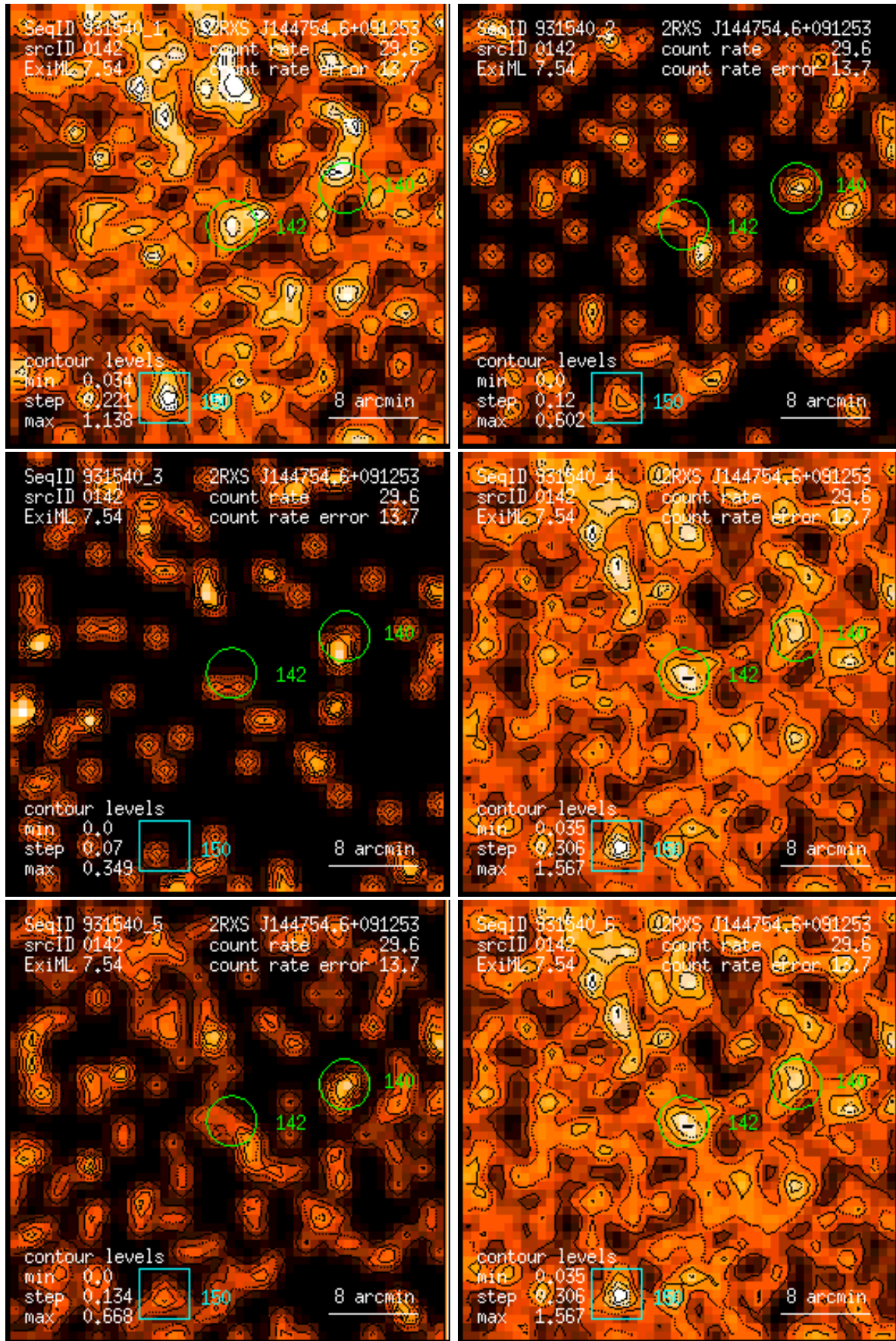
Figure 142: RASS 931540: detection 0142: band rate images, Gaussian filter: (1) PSPC channels 11 – 41, (2) 52 – 90, (3) 91 – 201, (4) 11 – 235, (5) 52 – 201, (6) 11 – 201. Broad band rates in counts/ks. Band rate contour levels in counts/ks/arcmin 2 .
