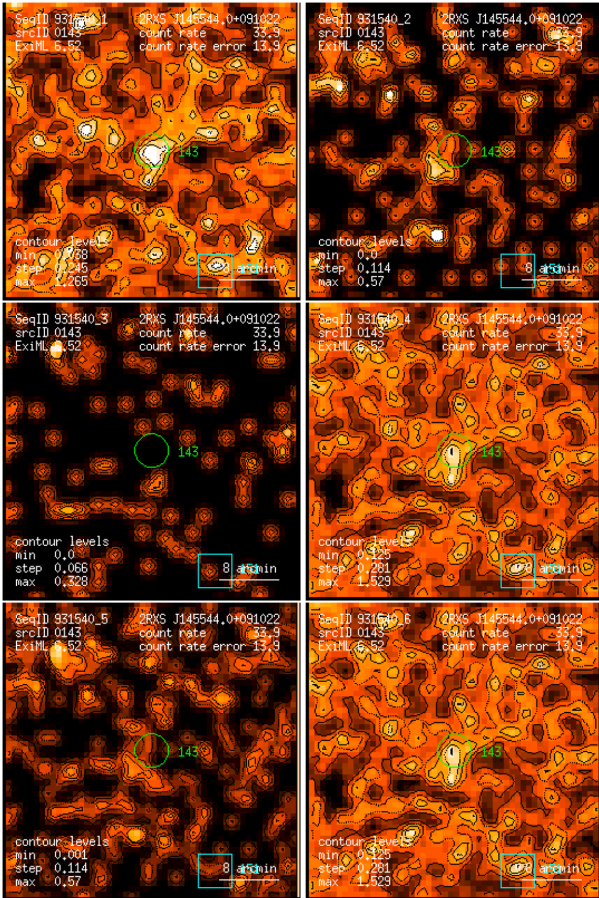
Figure 143: RASS 931540: detection 0143: band rate images, Gaussian filter: (1) PSPC channels 11 – 41, (2) 52 – 90, (3) 91 – 201, (4) 11 – 235, (5) 52 – 201, (6) 11 – 201. Broad band rates in counts/ks. Band rate contour levels in counts/ks/arcmin 2 .
