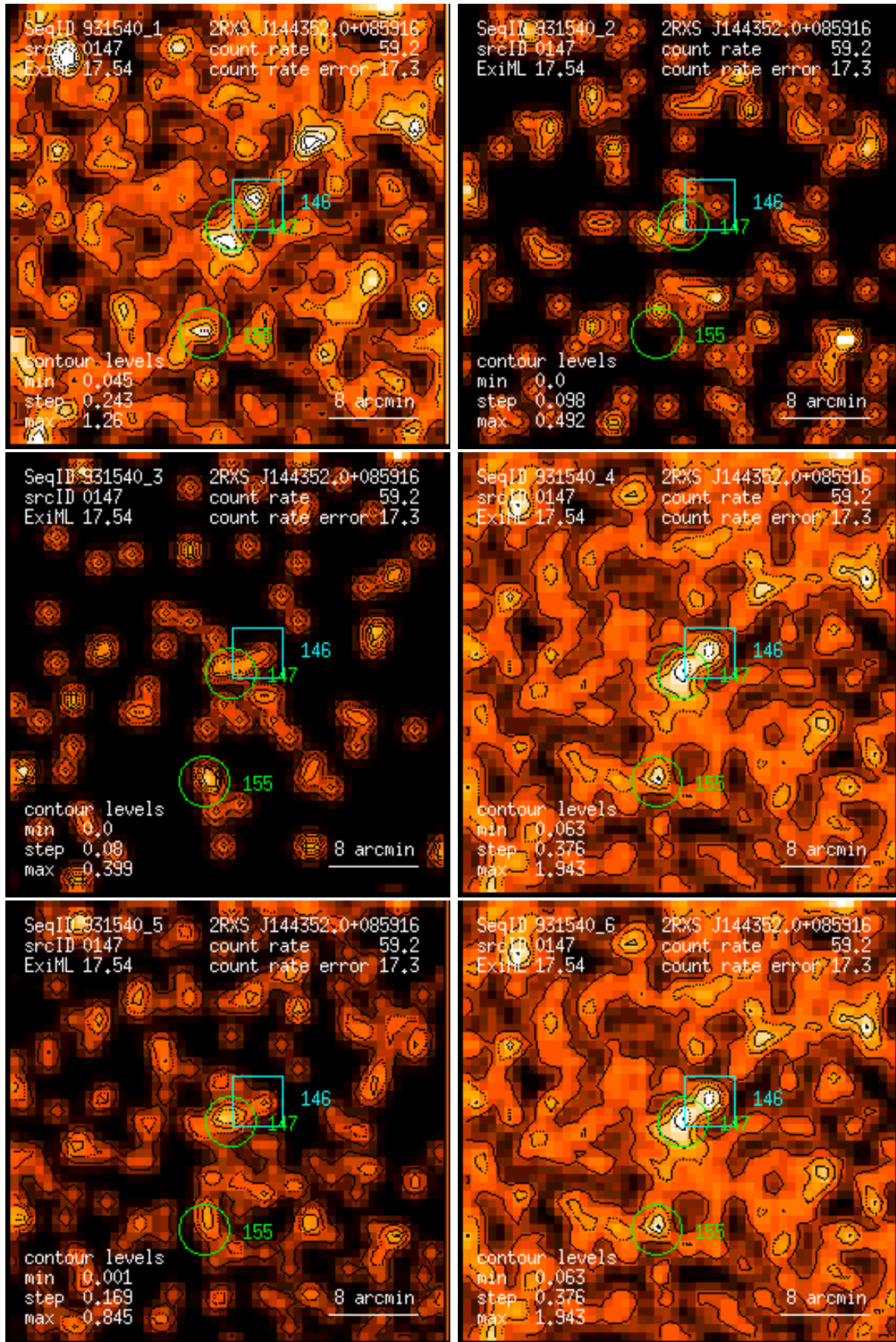
Figure 147: RASS 931540: detection 0147: band rate images, Gaussian filter: (1) PSPC channels 11 – 41, (2) 52 – 90, (3) 91 – 201, (4) 11 – 235, (5) 52 – 201, (6) 11 – 201. Broad band rates in counts/ks. Band rate contour levels in counts/ks/arcmin 2 .
