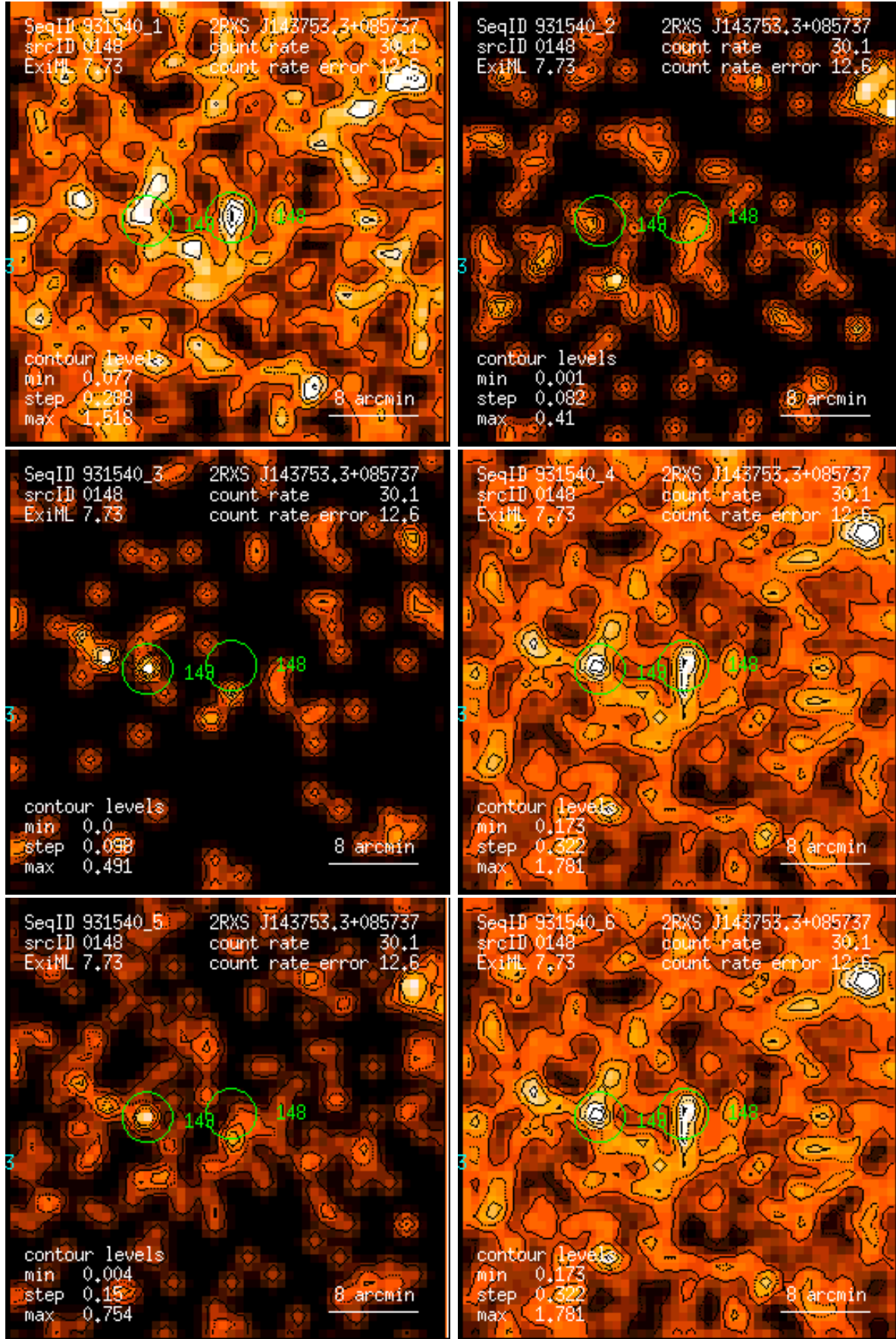
Figure 148: RASS 931540: detection 0148: band rate images, Gaussian filter: (1) PSPC channels 11 – 41, (2) 52 – 90, (3) 91 – 201, (4) 11 – 235, (5) 52 – 201, (6) 11 – 201. Broad band rates in counts/ks. Band rate contour levels in counts/ks/arcmin 2 .
