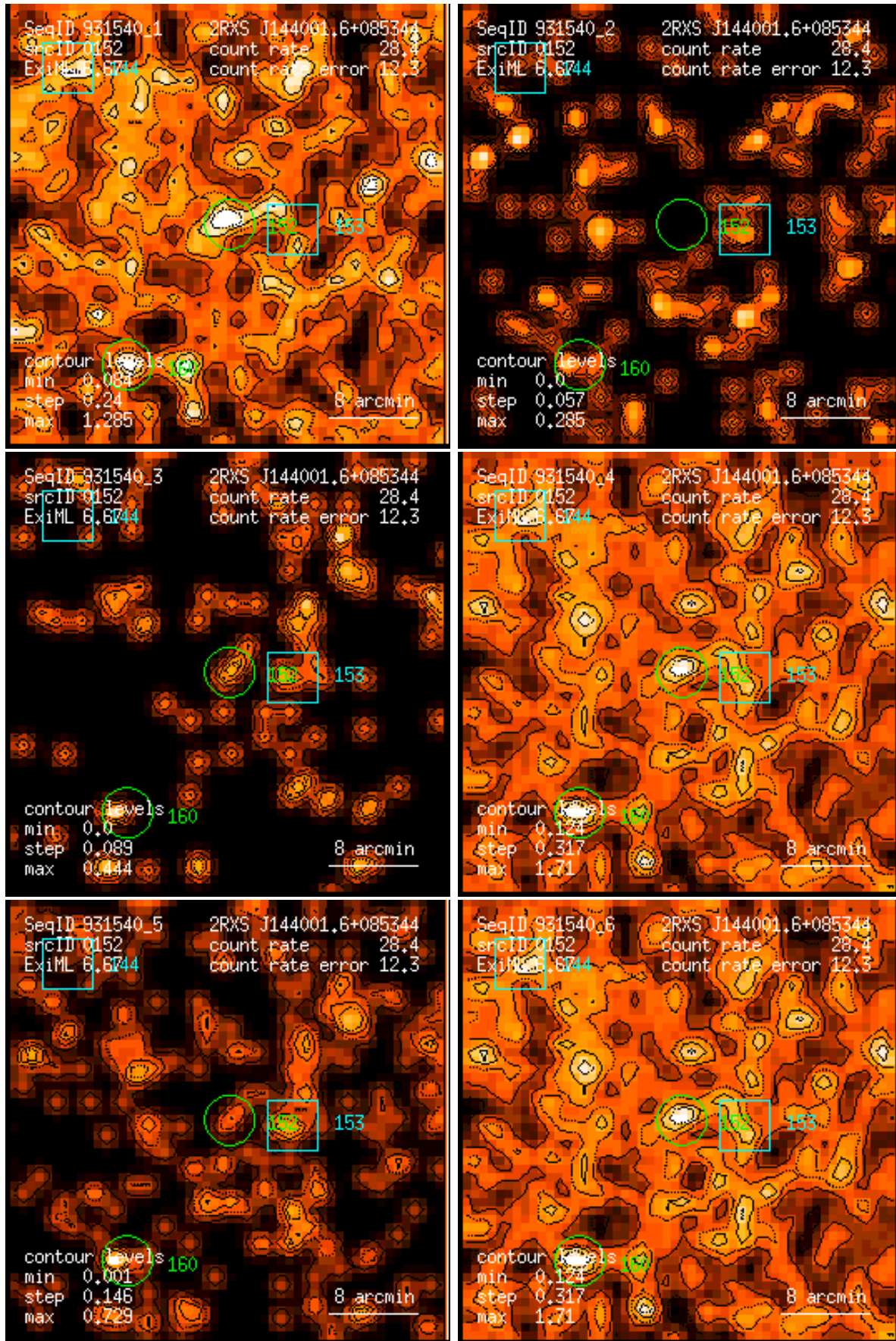
Figure 152: RASS 931540: detection 0152: band rate images, Gaussian filter: (1) PSPC channels 11 – 41, (2) 52 – 90, (3) 91 – 201, (4) 11 – 235, (5) 52 – 201, (6) 11 – 201. Broad band rates in counts/ks. Band rate contour levels in counts/ks/arcmin 2 .
