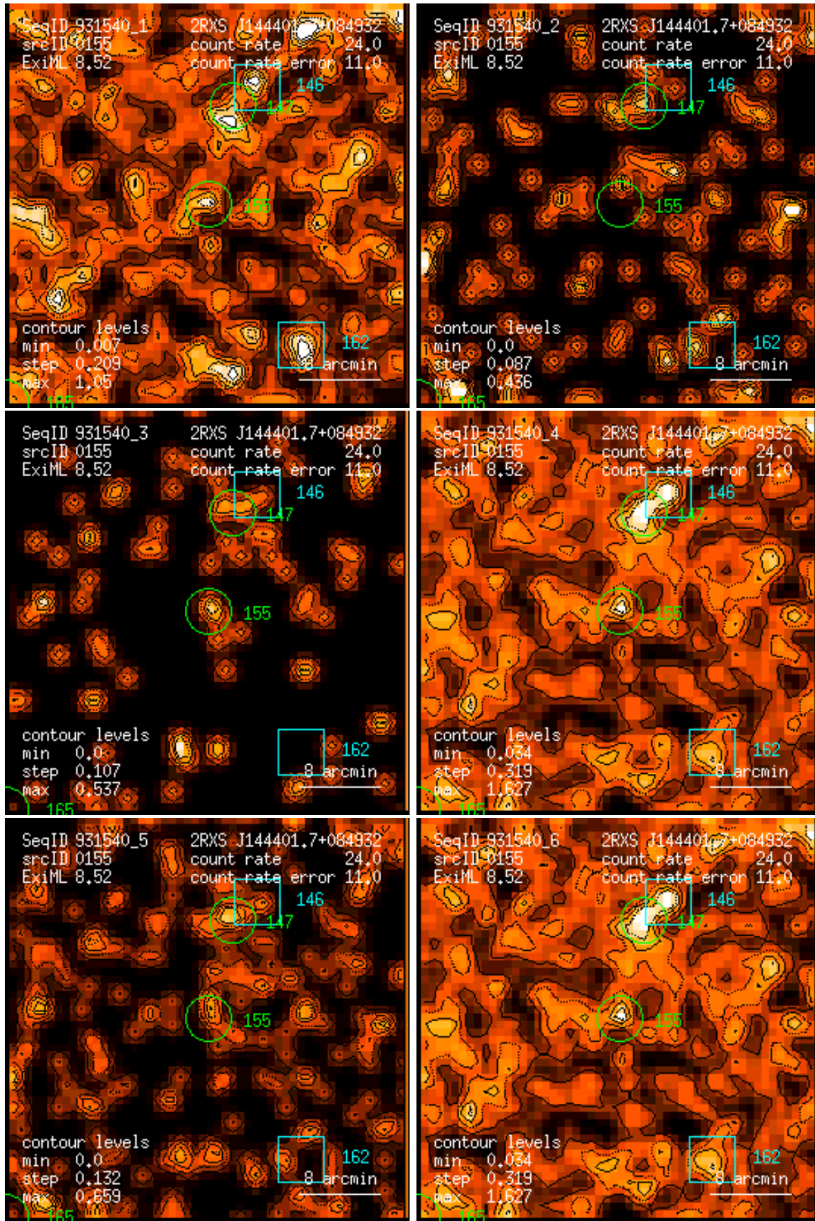
Figure 155: RASS 931540: detection 0155: band rate images, Gaussian filter: (1) PSPC channels 11 – 41, (2) 52 – 90, (3) 91 – 201, (4) 11 – 235, (5) 52 – 201, (6) 11 – 201. Broad band rates in counts/ks. Band rate contour levels in counts/ks/arcmin 2 .
