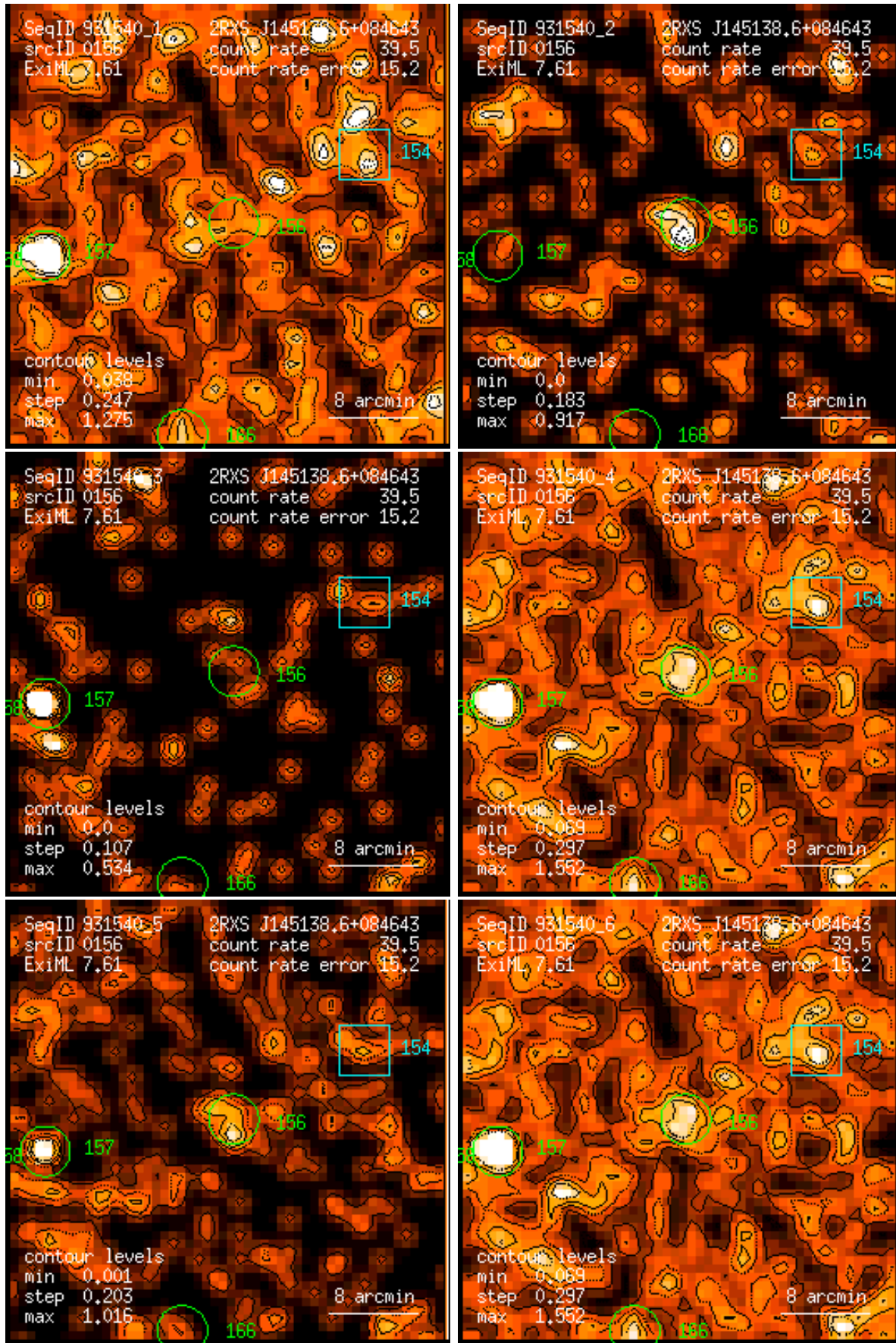
Figure 156: RASS 931540: detection 0156: band rate images, Gaussian filter: (1) PSPC channels 11 – 41, (2) 52 – 90, (3) 91 – 201, (4) 11 – 235, (5) 52 – 201, (6) 11 – 201. Broad band rates in counts/ks. Band rate contour levels in counts/ks/arcmin 2 .
