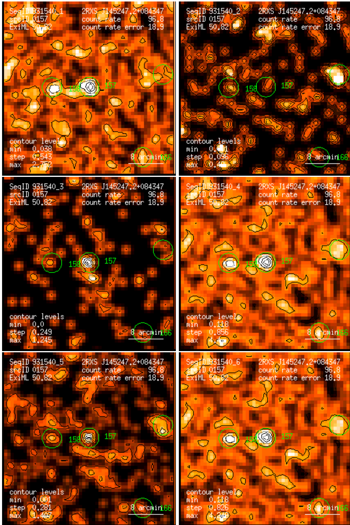
Figure 157: RASS 931540: detection 0157: band rate images, Gaussian filter: (1) PSPC channels 11 – 41, (2) 52 – 90, (3) 91 – 201, (4) 11 – 235, (5) 52 – 201, (6) 11 – 201. Broad band rates in counts/ks. Band rate contour levels in counts/ks/arcmin 2 .
