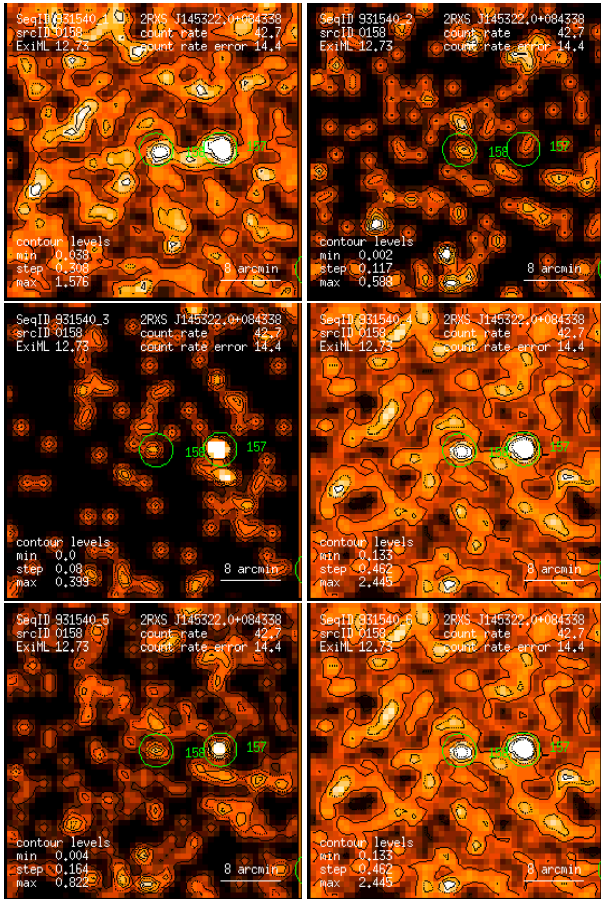
Figure 158: RASS 931540: detection 0158: band rate images, Gaussian filter: (1) PSPC channels 11 – 41, (2) 52 – 90, (3) 91 – 201, (4) 11 – 235, (5) 52 – 201, (6) 11 – 201. Broad band rates in counts/ks. Band rate contour levels in counts/ks/arcmin 2 .
