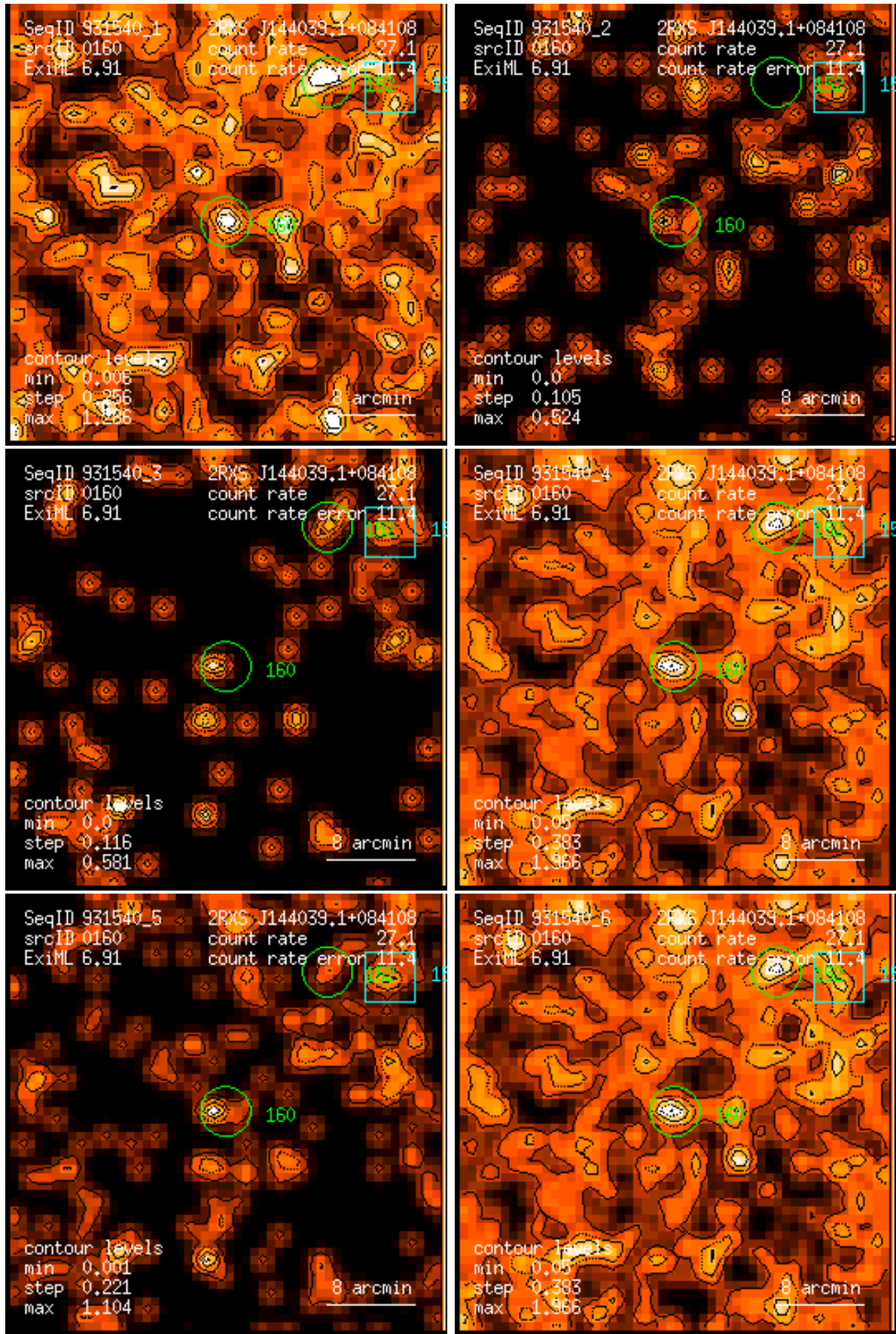
Figure 160: RASS 931540: detection 0160: band rate images, Gaussian filter: (1) PSPC channels 11 – 41, (2) 52 – 90, (3) 91 – 201, (4) 11 – 235, (5) 52 – 201, (6) 11 – 201. Broad band rates in counts/ks. Band rate contour levels in counts/ks/arcmin 2 .
