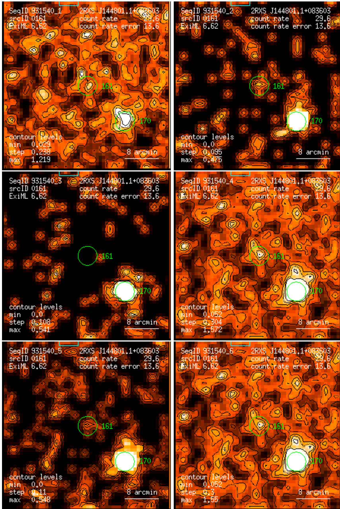
Figure 161: RASS 931540: detection 0161: band rate images, Gaussian filter: (1) PSPC channels 11 – 41, (2) 52 – 90, (3) 91 – 201, (4) 11 – 235, (5) 52 – 201, (6) 11 – 201. Broad band rates in counts/ks. Band rate contour levels in counts/ks/arcmin 2 .
