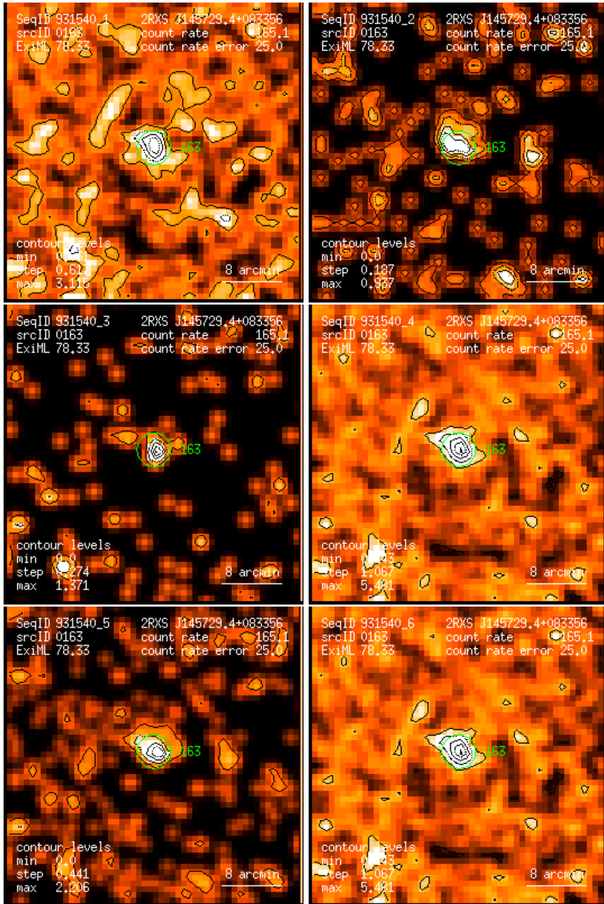
Figure 163: RASS 931540: detection 0163: band rate images, Gaussian filter: (1) PSPC channels 11 – 41, (2) 52 – 90, (3) 91 – 201, (4) 11 – 235, (5) 52 – 201, (6) 11 – 201. Broad band rates in counts/ks. Band rate contour levels in counts/ks/arcmin 2 .
