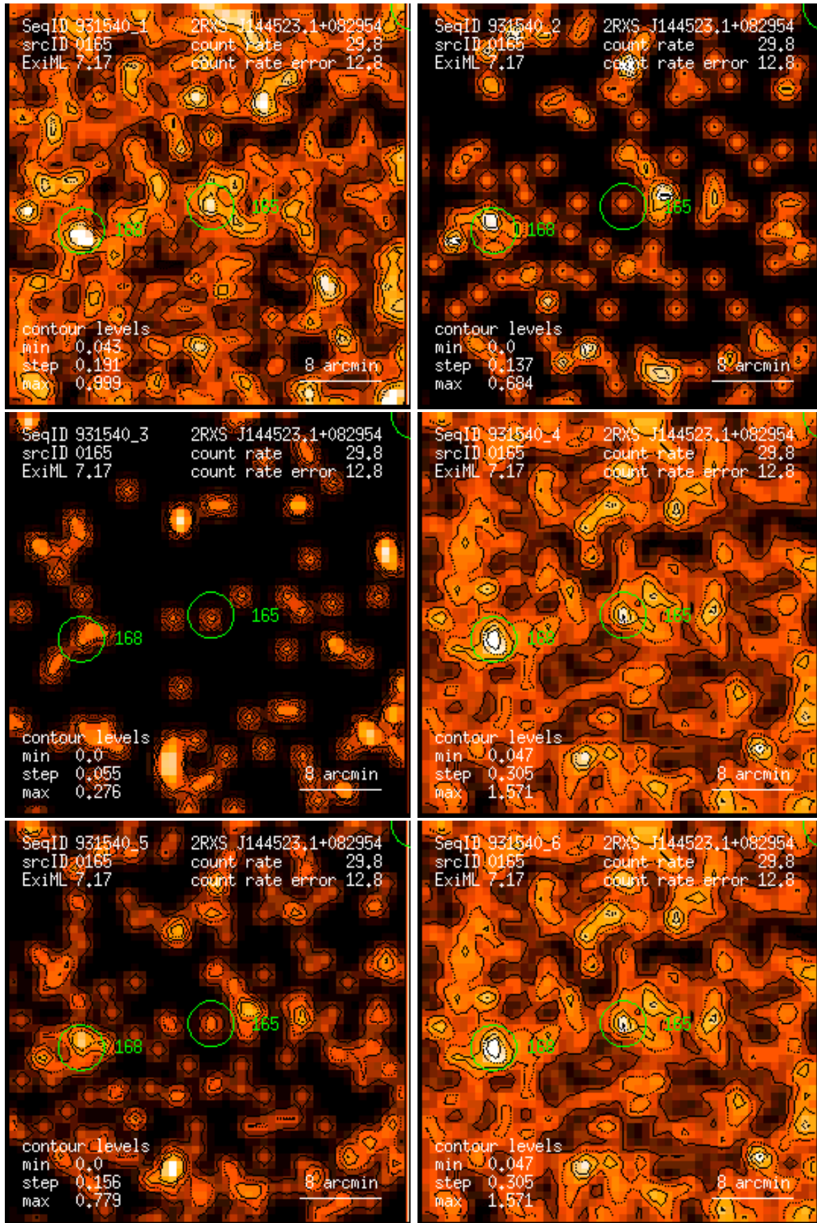
Figure 165: RASS 931540: detection 0165: band rate images, Gaussian filter: (1) PSPC channels 11 – 41, (2) 52 – 90, (3) 91 – 201, (4) 11 – 235, (5) 52 – 201, (6) 11 – 201. Broad band rates in counts/ks. Band rate contour levels in counts/ks/arcmin 2 .
