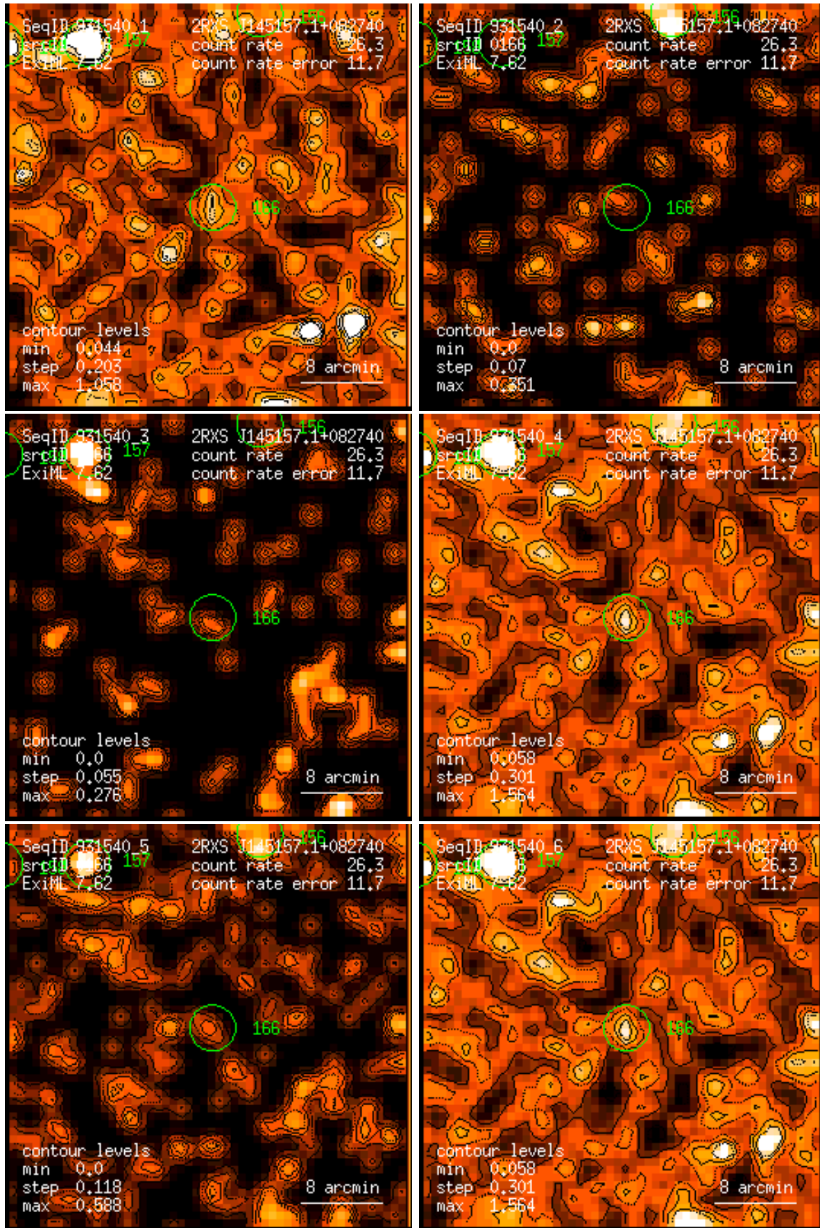
Figure 166: RASS 931540: detection 0166: band rate images, Gaussian filter: (1) PSPC channels 11 – 41, (2) 52 – 90, (3) 91 – 201, (4) 11 – 235, (5) 52 – 201, (6) 11 – 201. Broad band rates in counts/ks. Band rate contour levels in counts/ks/arcmin 2 .
