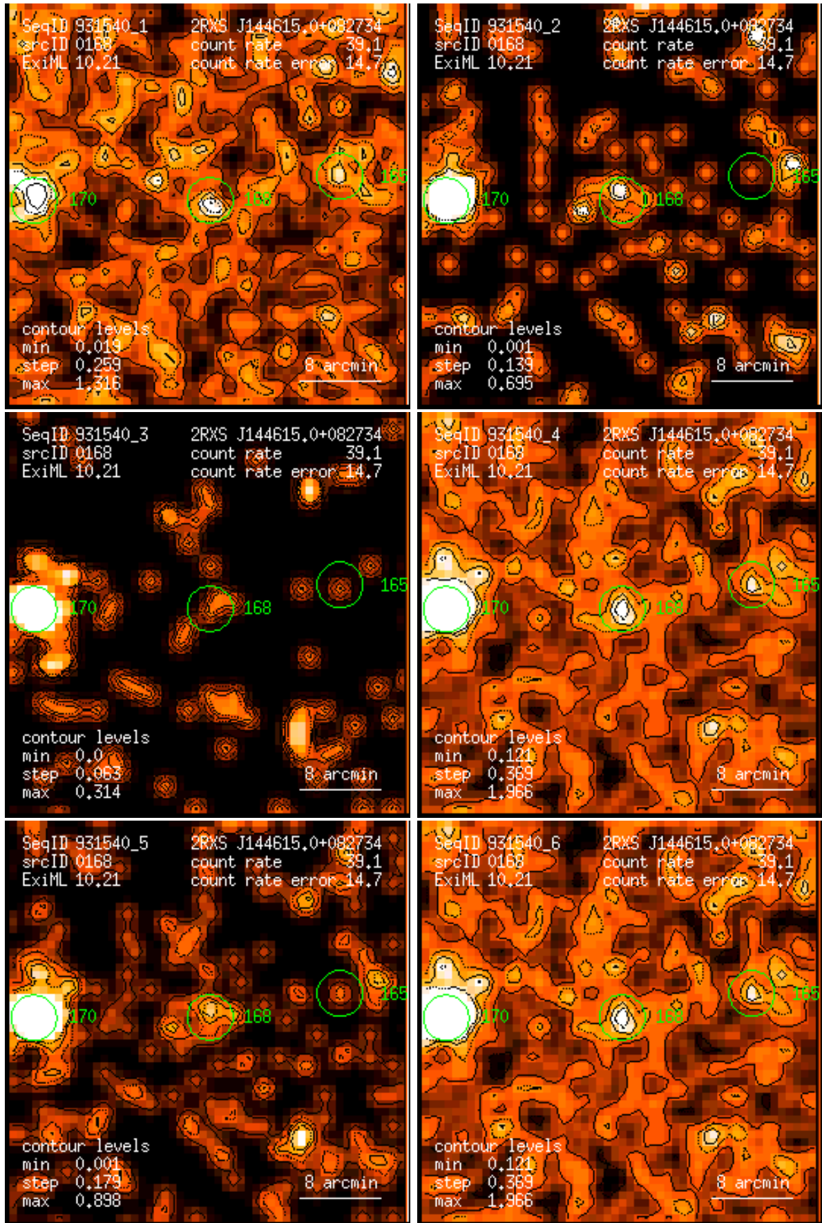
Figure 168: RASS 931540: detection 0168: band rate images, Gaussian filter: (1) PSPC channels 11 – 41, (2) 52 – 90, (3) 91 – 201, (4) 11 – 235, (5) 52 – 201, (6) 11 – 201. Broad band rates in counts/ks. Band rate contour levels in counts/ks/arcmin 2 .
