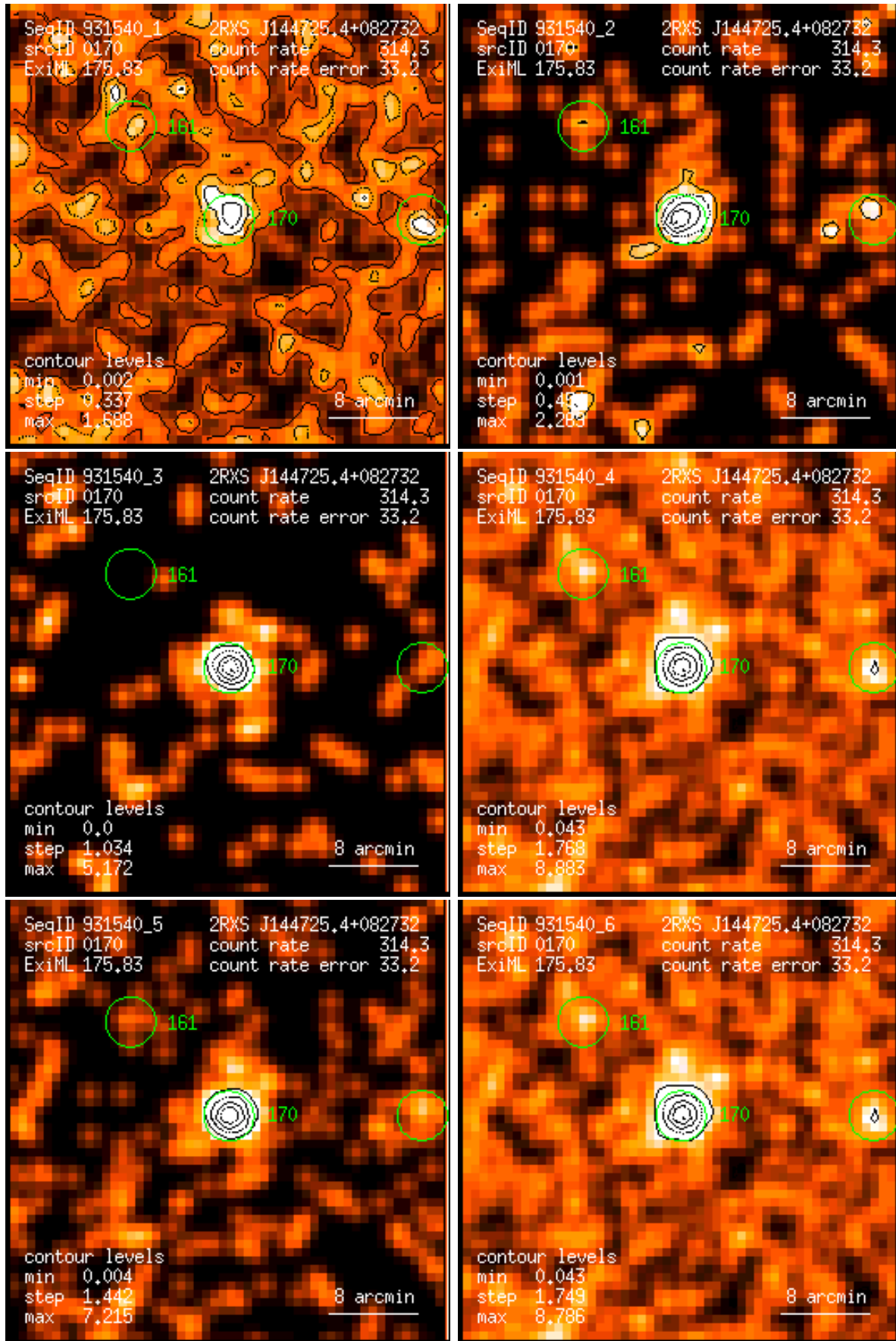
Figure 170: RASS 931540: detection 0170: band rate images, Gaussian filter: (1) PSPC channels 11 – 41, (2) 52 – 90, (3) 91 – 201, (4) 11 – 235, (5) 52 – 201, (6) 11 – 201. Broad band rates in counts/ks. Band rate contour levels in counts/ks/arcmin 2 .
