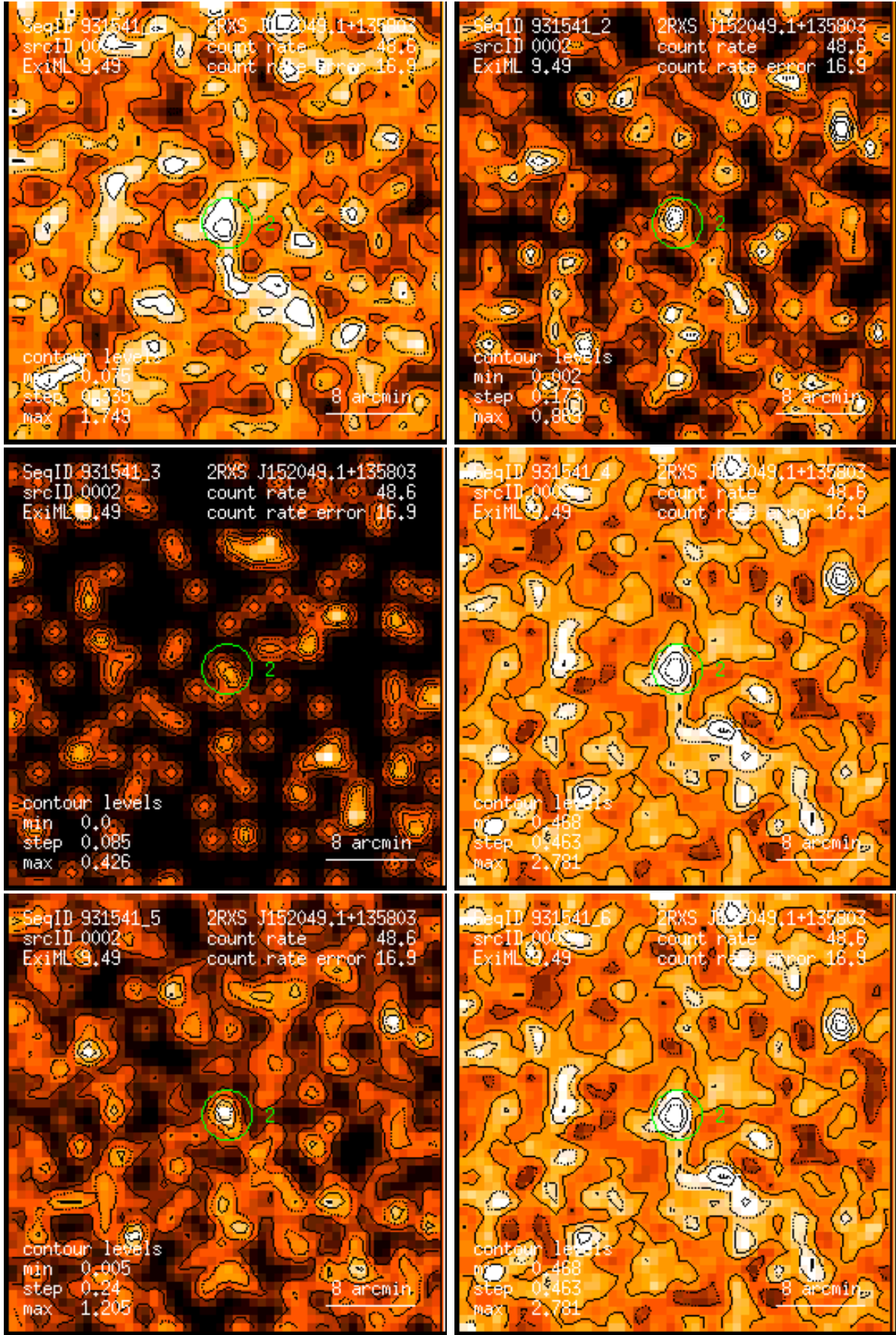
Figure 2: RASS 931541: detection 0002: band rate images, Gaussian filter: (1) PSPC channels 11 – 41, (2) 52 – 90, (3) 91 – 201, (4) 11 – 235, (5) 52 – 201, (6) 11 – 201. Broad band rates in counts/ks. Band rate contour levels in counts/ks/arcmin 2 .
