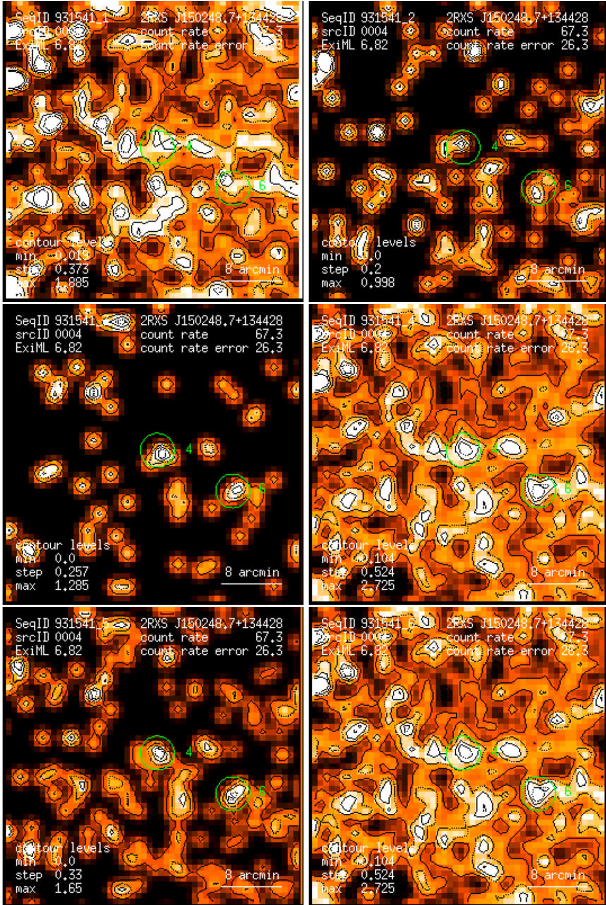
Figure 4: RASS 931541: detection 0004: band rate images, Gaussian filter: (1) PSPC channels 11 – 41, (2) 52 – 90, (3) 91 – 201, (4) 11 – 235, (5) 52 – 201, (6) 11 – 201. Broad band rates in counts/ks. Band rate contour levels in counts/ks/arcmin 2 .
