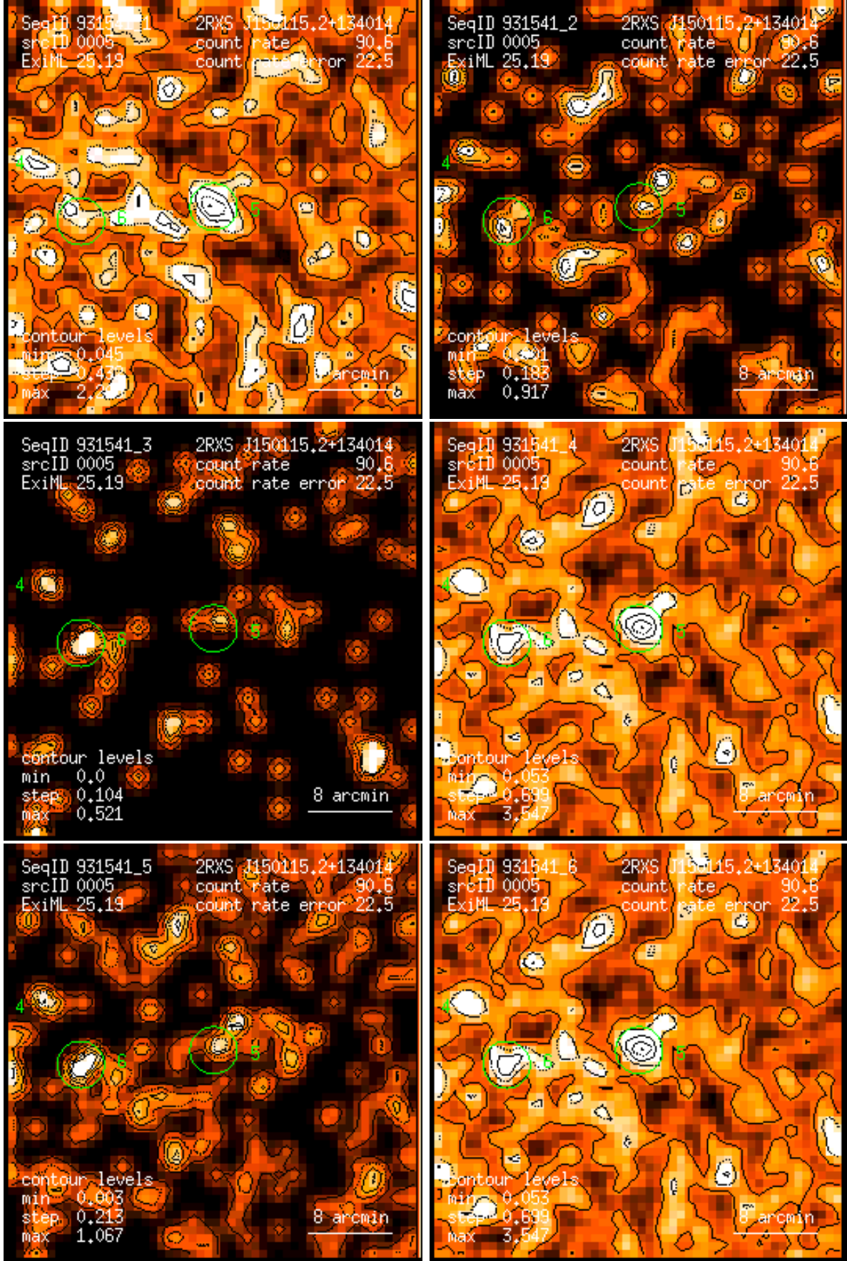
Figure 5: RASS 931541: detection 0005: band rate images, Gaussian filter: (1) PSPC channels 11 – 41, (2) 52 – 90, (3) 91 – 201, (4) 11 – 235, (5) 52 – 201, (6) 11 – 201. Broad band rates in counts/ks. Band rate contour levels in counts/ks/arcmin 2 .
