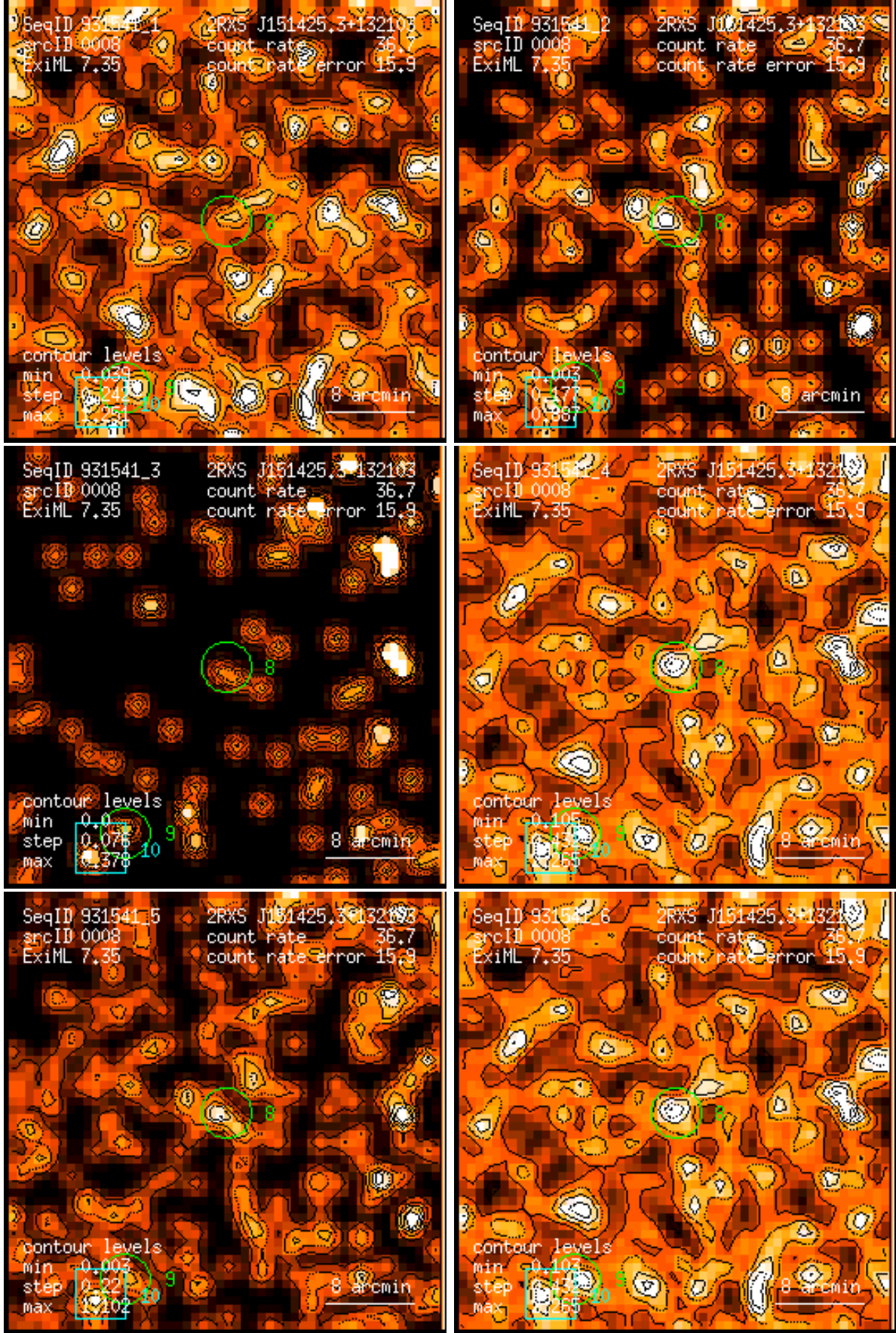
Figure 8: RASS 931541: detection 0008: band rate images, Gaussian filter: (1) PSPC channels 11 – 41, (2) 52 – 90, (3) 91 – 201, (4) 11 – 235, (5) 52 – 201, (6) 11 – 201. Broad band rates in counts/ks. Band rate contour levels in counts/ks/arcmin 2 .
