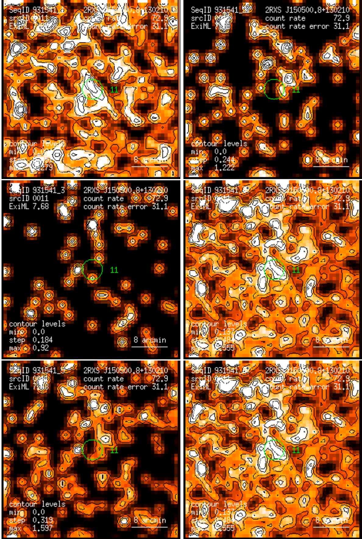
Figure 11: RASS 931541: detection 0011: band rate images, Gaussian filter: (1) PSPC channels 11 – 41, (2) 52 – 90, (3) 91 – 201, (4) 11 – 235, (5) 52 – 201, (6) 11 – 201. Broad band rates in counts/ks. Band rate contour levels in counts/ks/arcmin 2 .
