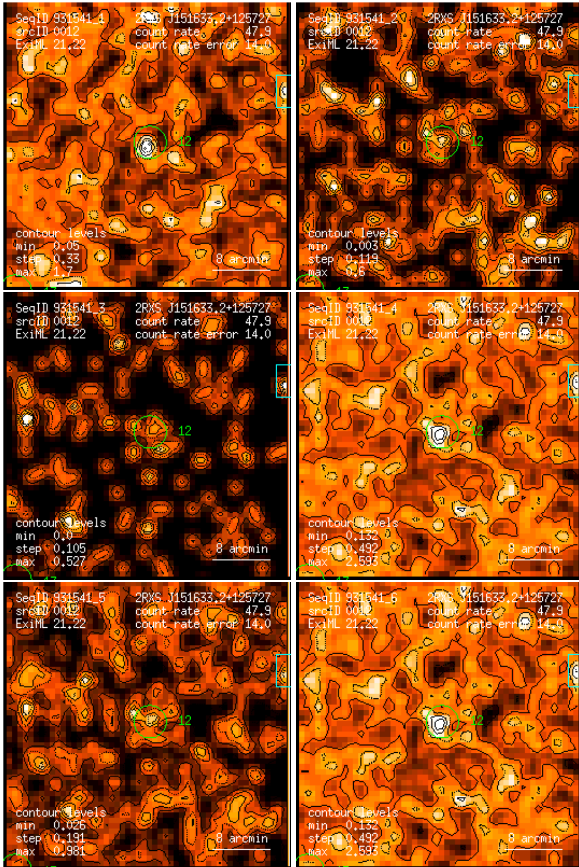
Figure 12: RASS 931541: detection 0012: band rate images, Gaussian filter: (1) PSPC channels 11 – 41, (2) 52 – 90, (3) 91 – 201, (4) 11 – 235, (5) 52 – 201, (6) 11 – 201. Broad band rates in counts/ks. Band rate contour levels in counts/ks/arcmin 2 .
