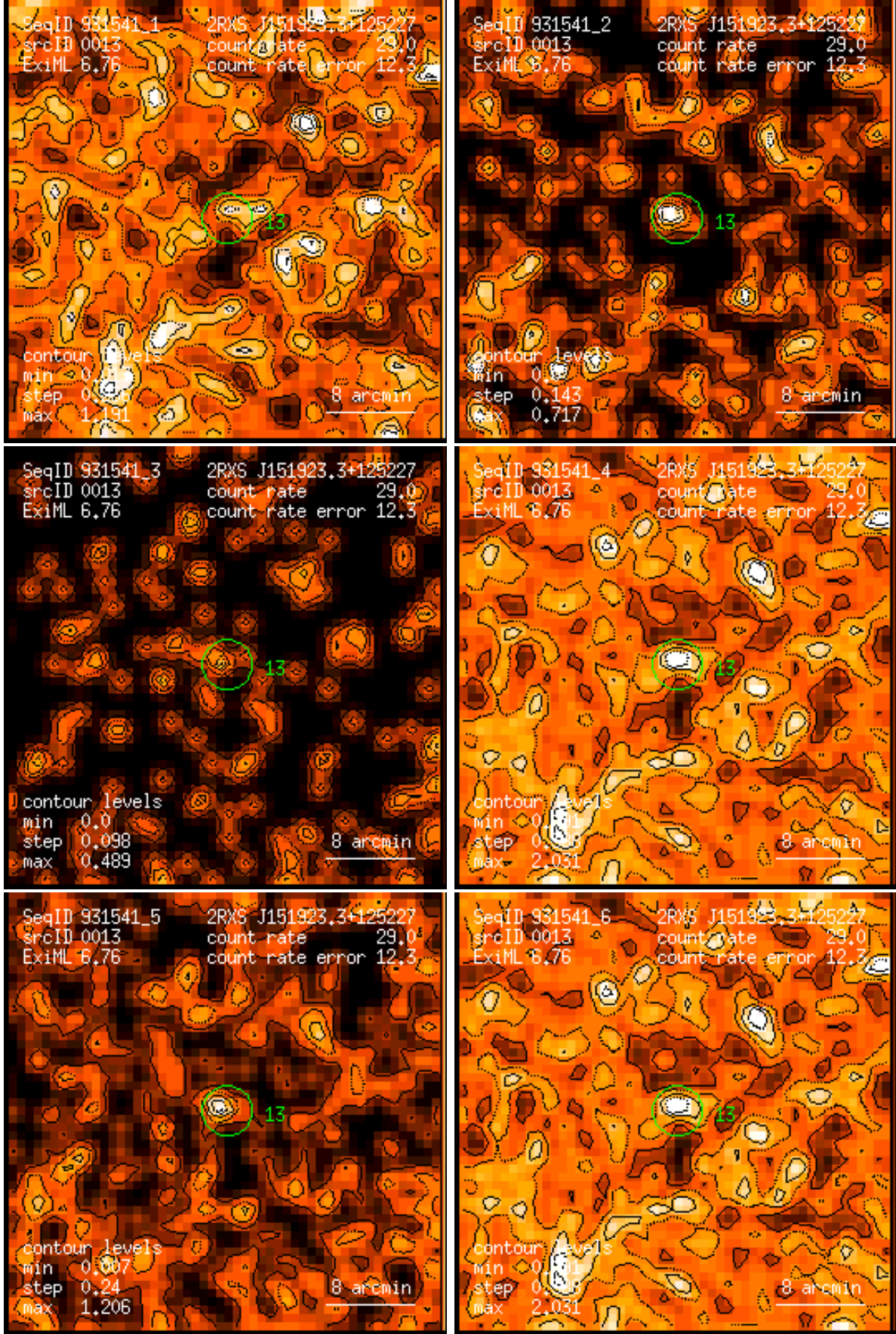
Figure 13: RASS 931541: detection 0013: band rate images, Gaussian filter: (1) PSPC channels 11 – 41, (2) 52 – 90, (3) 91 – 201, (4) 11 – 235, (5) 52 – 201, (6) 11 – 201. Broad band rates in counts/ks. Band rate contour levels in counts/ks/arcmin 2 .
