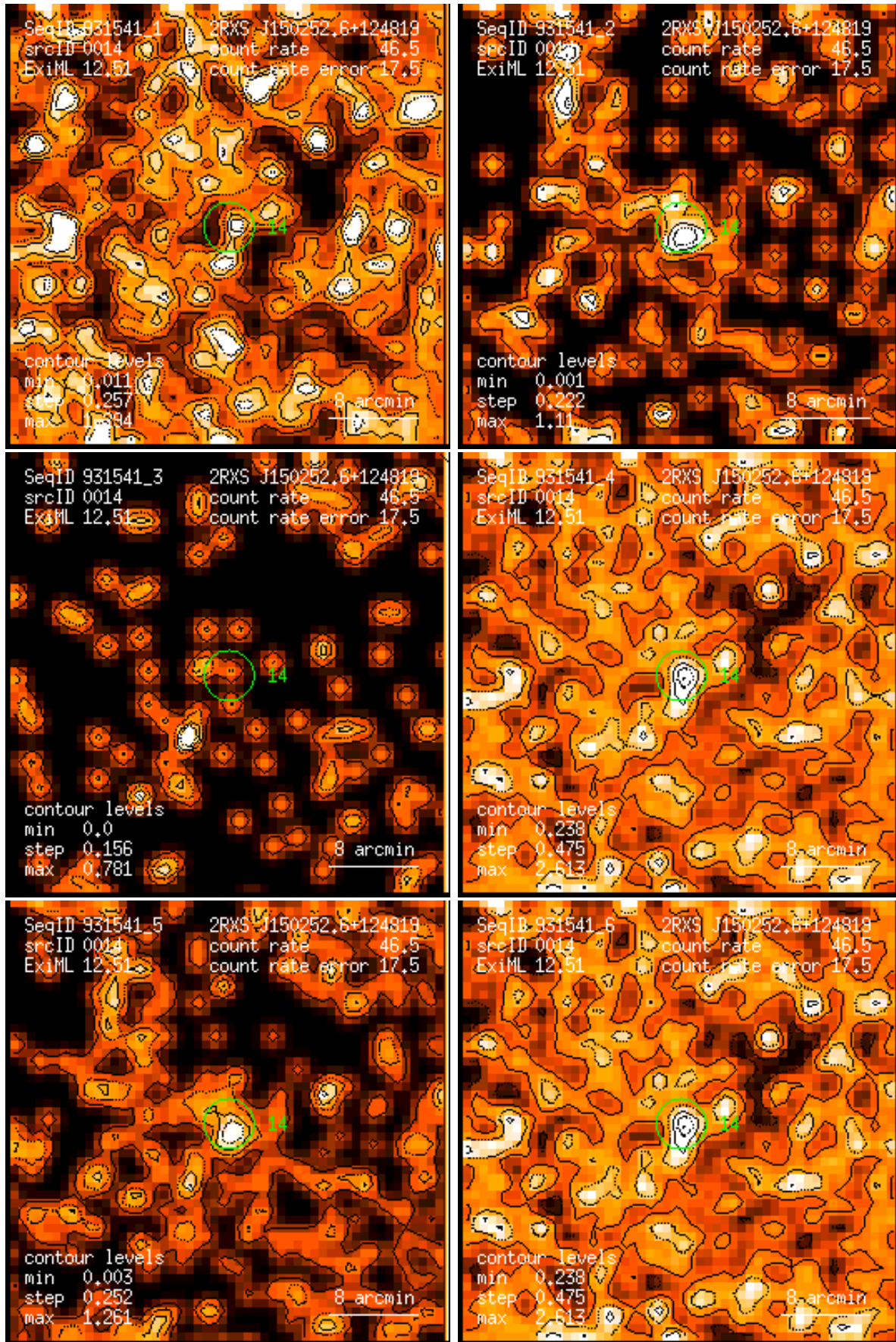
Figure 14: RASS 931541: detection 0014: band rate images, Gaussian filter: (1) PSPC channels 11 – 41, (2) 52 – 90, (3) 91 – 201, (4) 11 – 235, (5) 52 – 201, (6) 11 – 201. Broad band rates in counts/ks. Band rate contour levels in counts/ks/arcmin 2 .
