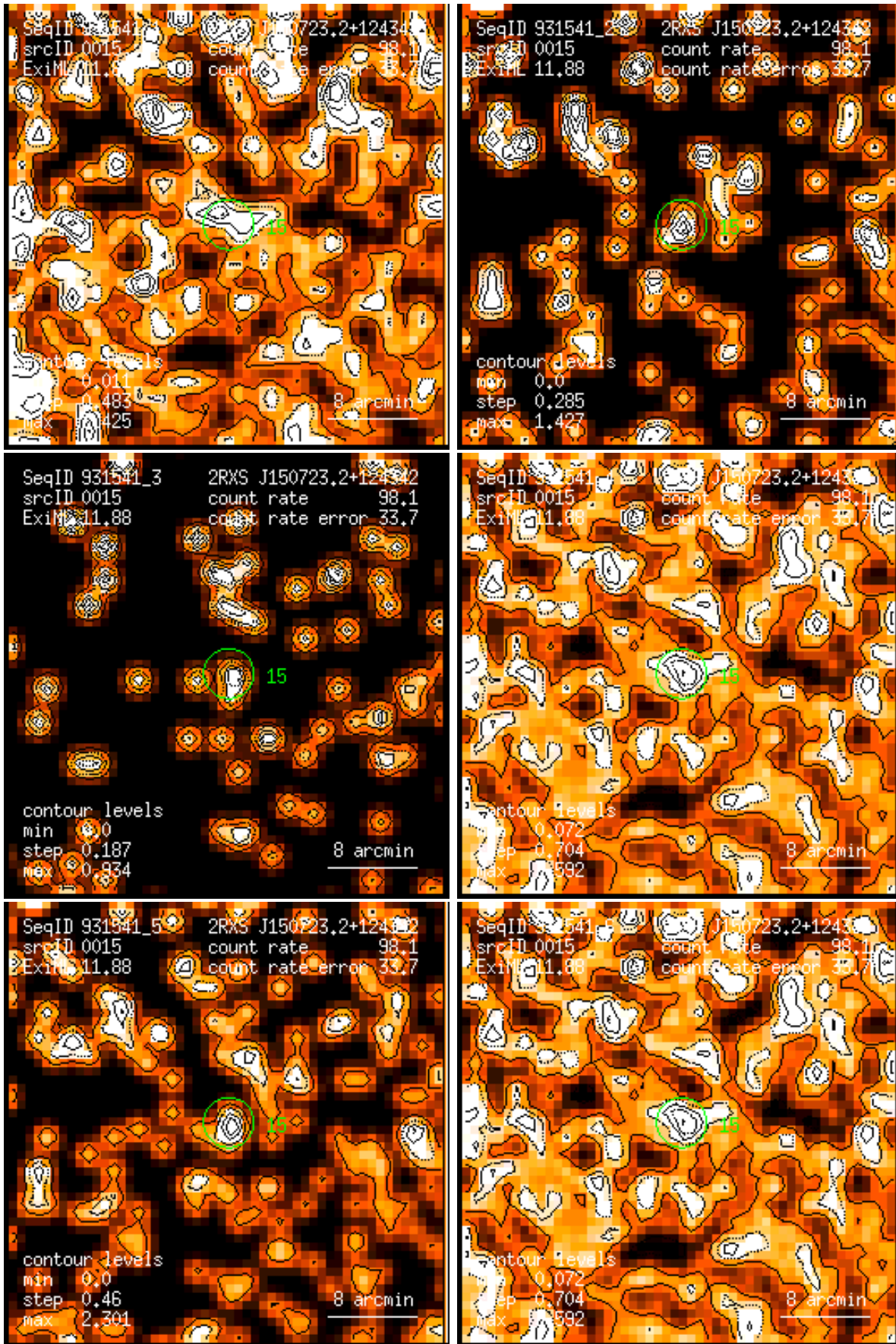
Figure 15: RASS 931541: detection 0015: band rate images, Gaussian filter: (1) PSPC channels 11 – 41, (2) 52 – 90, (3) 91 – 201, (4) 11 – 235, (5) 52 – 201, (6) 11 – 201. Broad band rates in counts/ks. Band rate contour levels in counts/ks/arcmin 2 .
