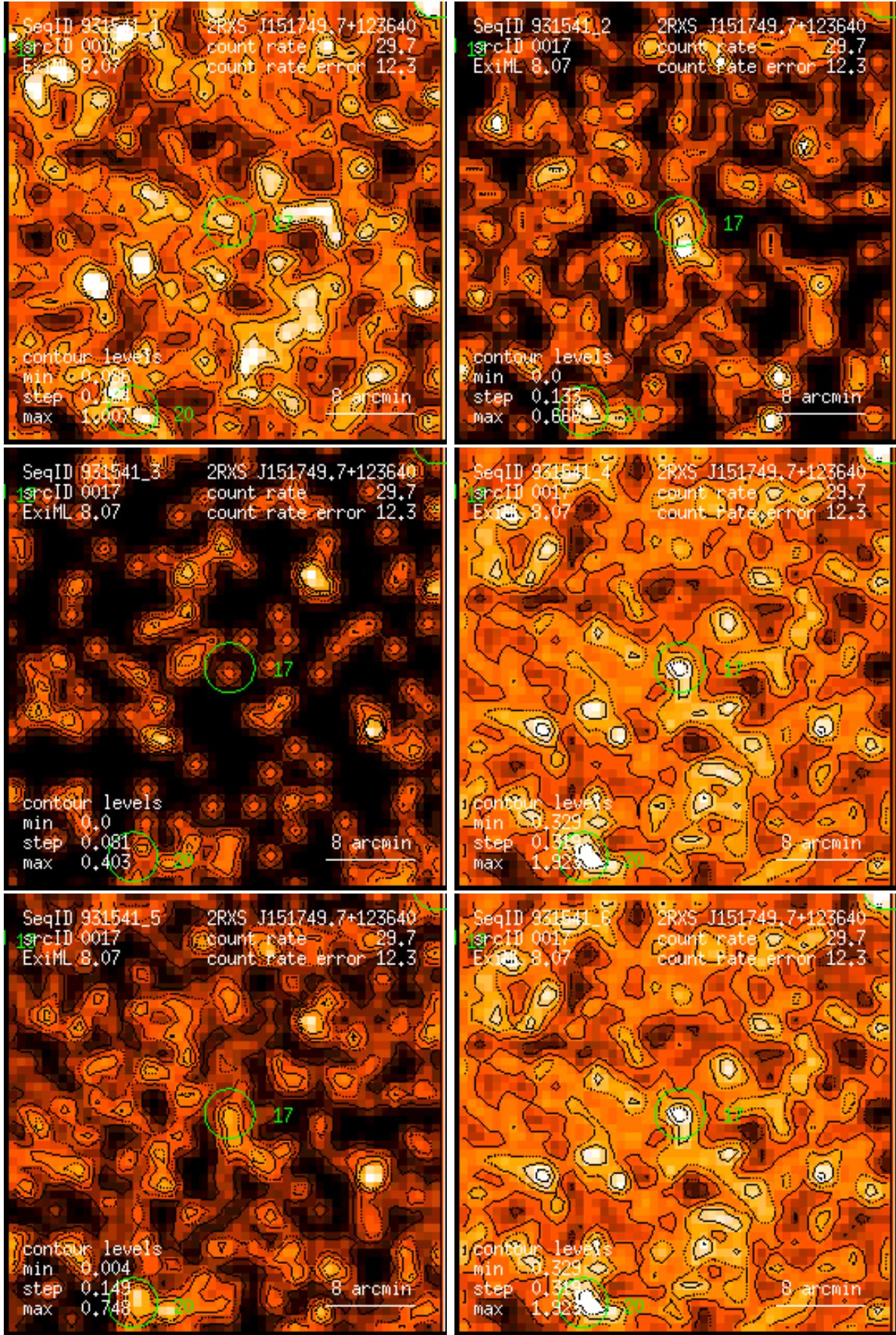
Figure 17: RASS 931541: detection 0017: band rate images, Gaussian filter: (1) PSPC channels 11 – 41, (2) 52 – 90, (3) 91 – 201, (4) 11 – 235, (5) 52 – 201, (6) 11 – 201. Broad band rates in counts/ks. Band rate contour levels in counts/ks/arcmin 2 .
