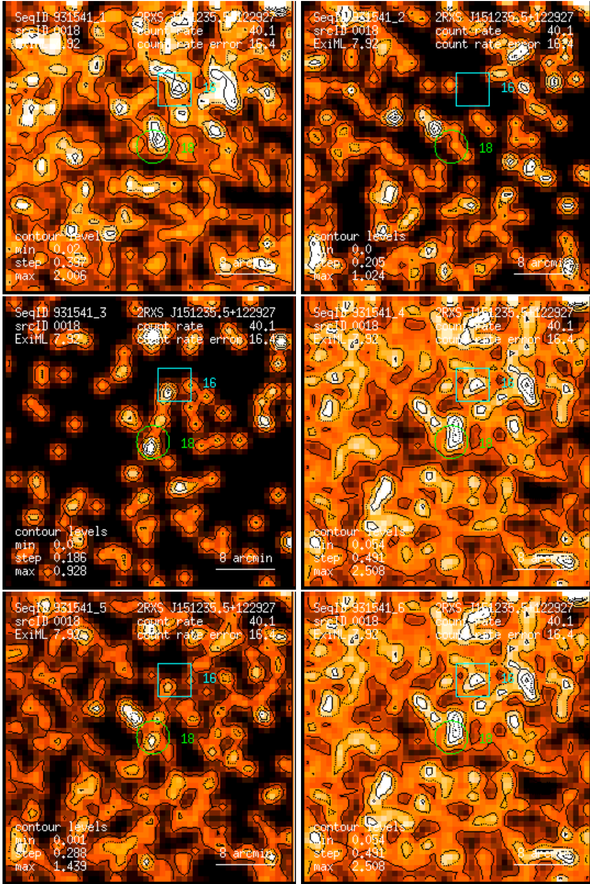
Figure 18: RASS 931541: detection 0018: band rate images, Gaussian filter: (1) PSPC channels 11 – 41, (2) 52 – 90, (3) 91 – 201, (4) 11 – 235, (5) 52 – 201, (6) 11 – 201. Broad band rates in counts/ks. Band rate contour levels in counts/ks/arcmin 2 .
