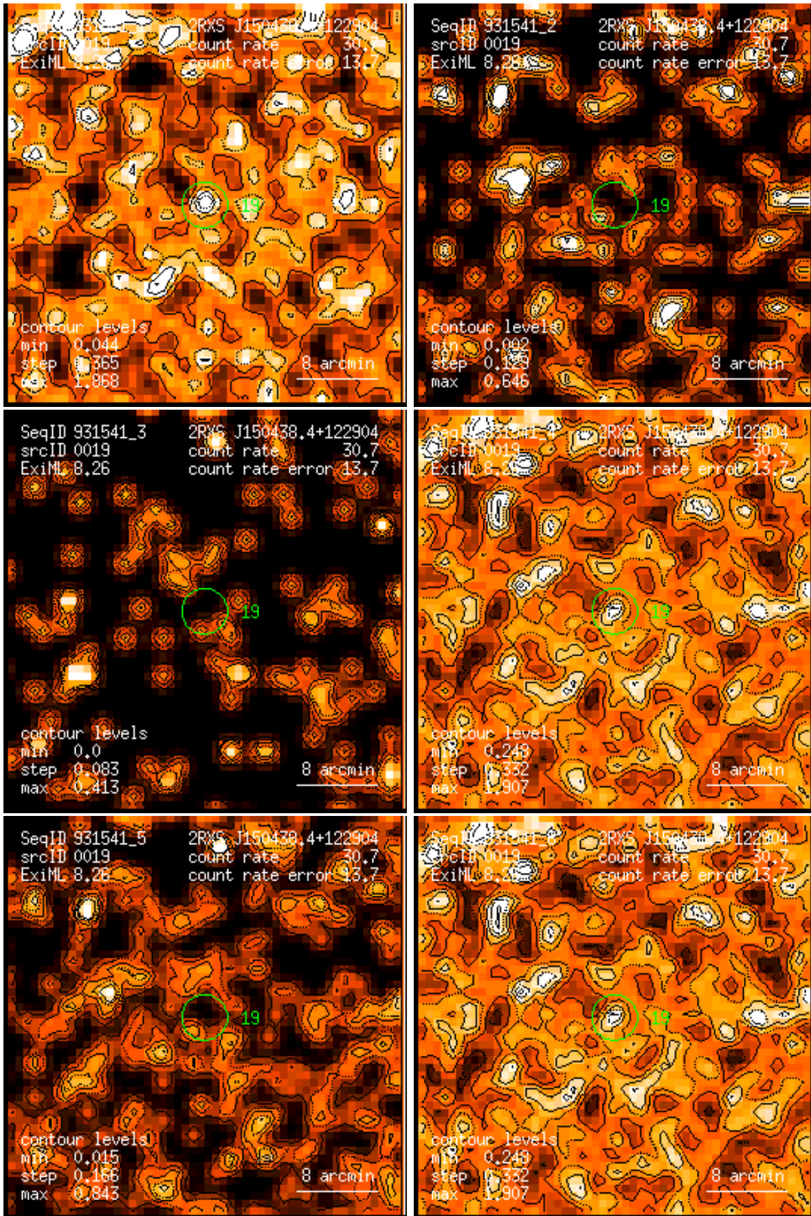
Figure 19: RASS 931541: detection 0019: band rate images, Gaussian filter: (1) PSPC channels 11 – 41, (2) 52 – 90, (3) 91 – 201, (4) 11 – 235, (5) 52 – 201, (6) 11 – 201. Broad band rates in counts/ks. Band rate contour levels in counts/ks/arcmin 2 .
