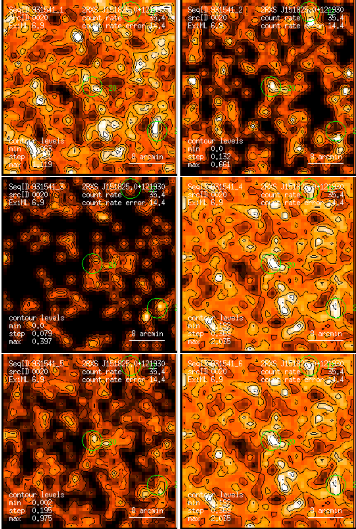
Figure 20: RASS 931541: detection 0020: band rate images, Gaussian filter: (1) PSPC channels 11 – 41, (2) 52 – 90, (3) 91 – 201, (4) 11 – 235, (5) 52 – 201, (6) 11 – 201. Broad band rates in counts/ks. Band rate contour levels in counts/ks/arcmin 2 .
