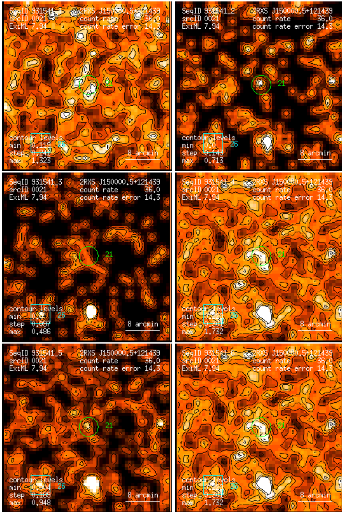
Figure 21: RASS 931541: detection 0021: band rate images, Gaussian filter: (1) PSPC channels 11 – 41, (2) 52 – 90, (3) 91 – 201, (4) 11 – 235, (5) 52 – 201, (6) 11 – 201. Broad band rates in counts/ks. Band rate contour levels in counts/ks/arcmin 2 .
