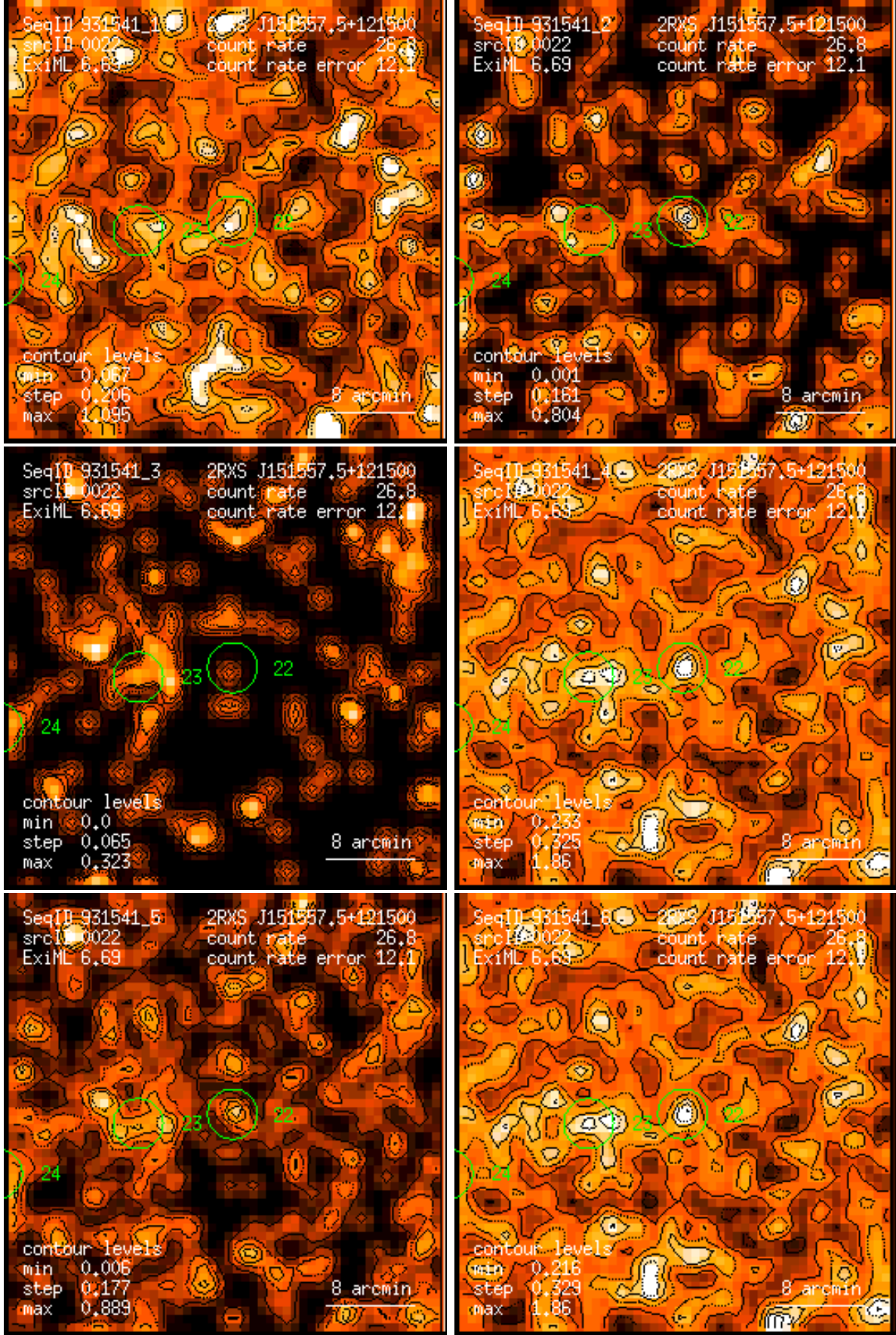
Figure 22: RASS 931541: detection 0022: band rate images, Gaussian filter: (1) PSPC channels 11 – 41, (2) 52 – 90, (3) 91 – 201, (4) 11 – 235, (5) 52 – 201, (6) 11 – 201. Broad band rates in counts/ks. Band rate contour levels in counts/ks/arcmin 2 .
