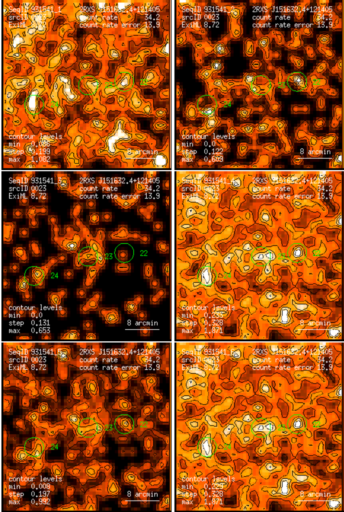
Figure 23: RASS 931541: detection 0023: band rate images, Gaussian filter: (1) PSPC channels 11 – 41, (2) 52 – 90, (3) 91 – 201, (4) 11 – 235, (5) 52 – 201, (6) 11 – 201. Broad band rates in counts/ks. Band rate contour levels in counts/ks/arcmin 2 .
