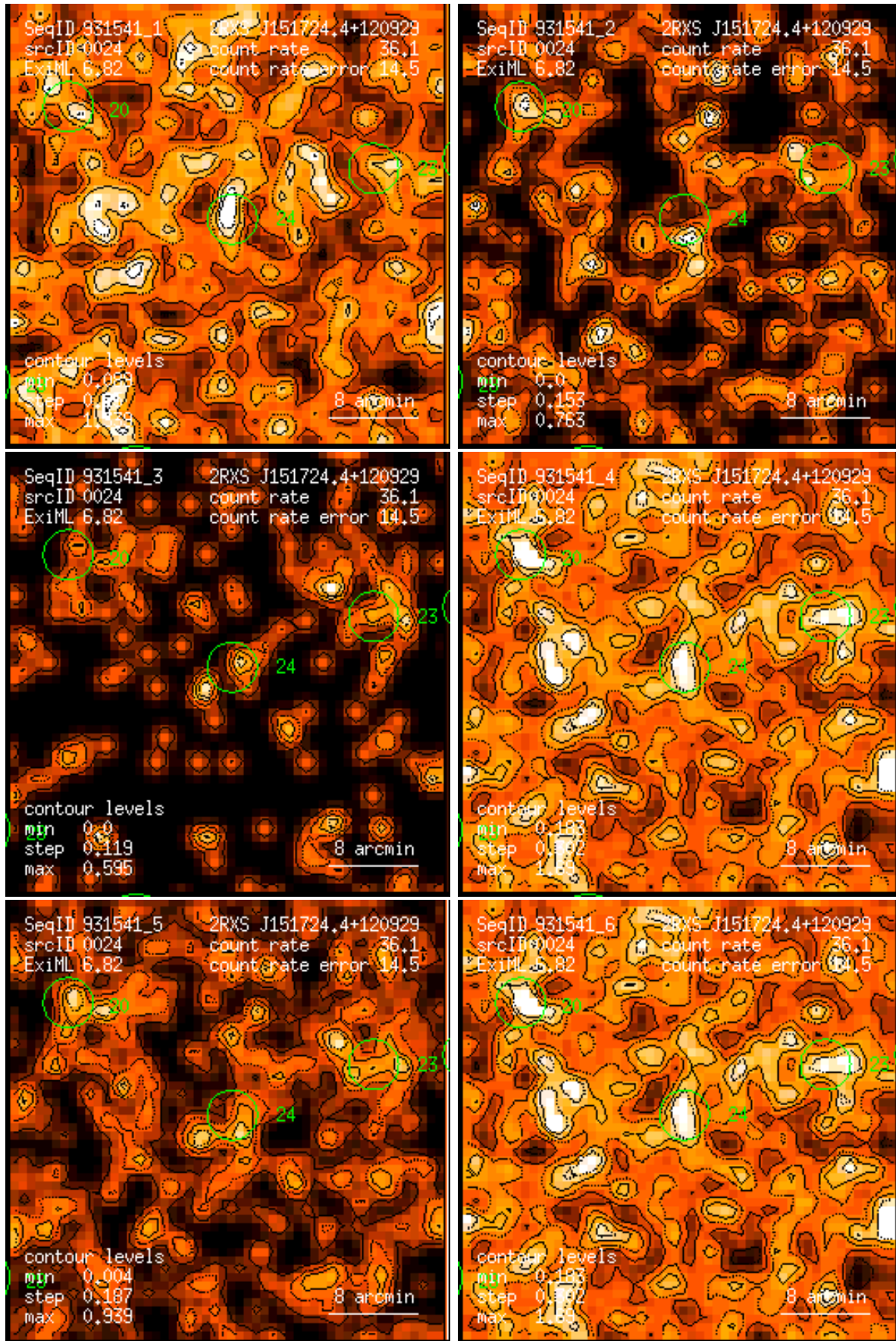
Figure 24: RASS 931541: detection 0024: band rate images, Gaussian filter: (1) PSPC channels 11 – 41, (2) 52 – 90, (3) 91 – 201, (4) 11 – 235, (5) 52 – 201, (6) 11 – 201. Broad band rates in counts/ks. Band rate contour levels in counts/ks/arcmin 2 .
