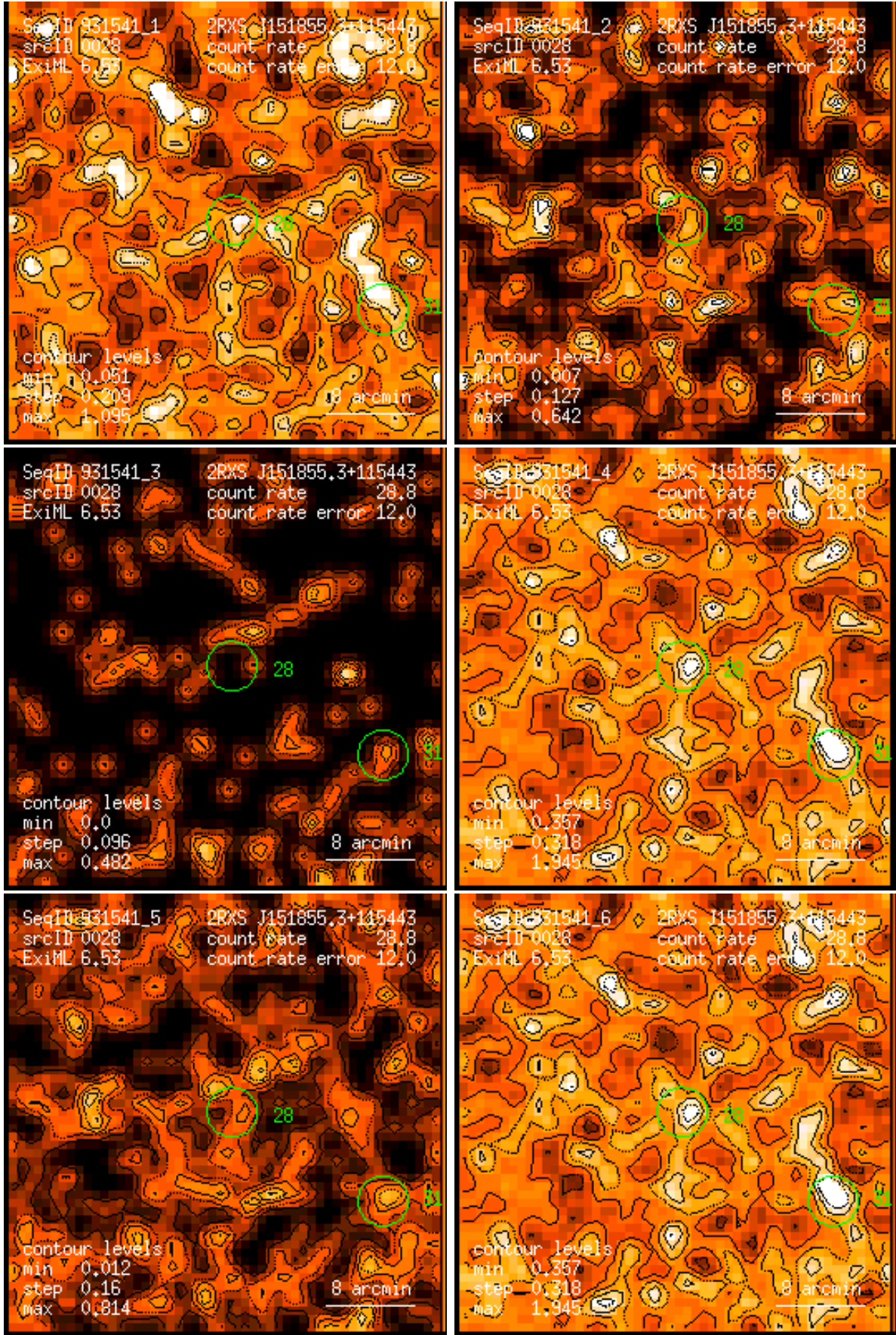
Figure 28: RASS 931541: detection 0028: band rate images, Gaussian filter: (1) PSPC channels 11 – 41, (2) 52 – 90, (3) 91 – 201, (4) 11 – 235, (5) 52 – 201, (6) 11 – 201. Broad band rates in counts/ks. Band rate contour levels in counts/ks/arcmin 2 .
