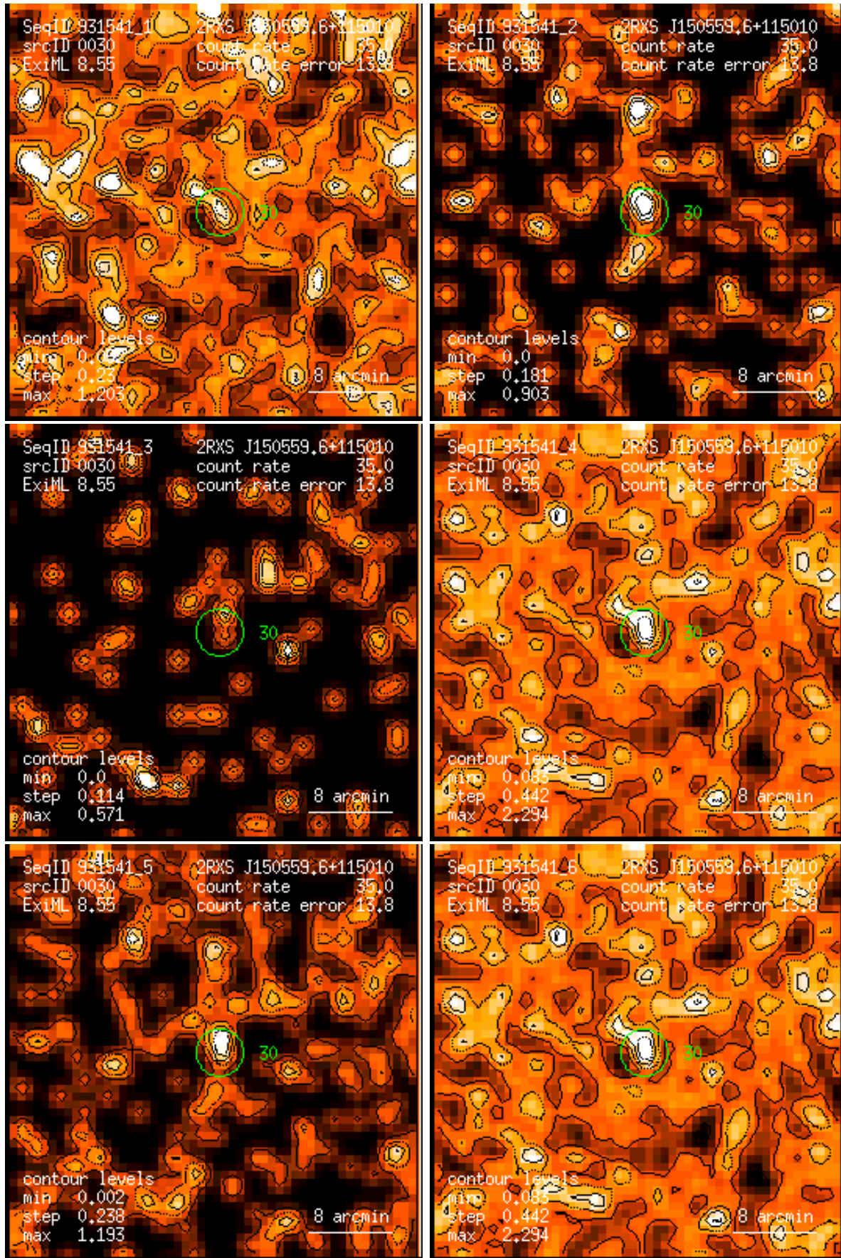
Figure 30: RASS 931541: detection 0030: band rate images, Gaussian filter: (1) PSPC channels 11 – 41, (2) 52 – 90, (3) 91 – 201, (4) 11 – 235, (5) 52 – 201, (6) 11 – 201. Broad band rates in counts/ks. Band rate contour levels in counts/ks/arcmin 2 .
