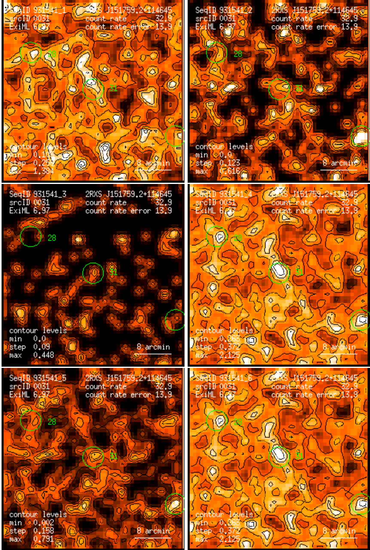
Figure 31: RASS 931541: detection 0031: band rate images, Gaussian filter: (1) PSPC channels 11 – 41, (2) 52 – 90, (3) 91 – 201, (4) 11 – 235, (5) 52 – 201, (6) 11 – 201. Broad band rates in counts/ks. Band rate contour levels in counts/ks/arcmin 2 .
