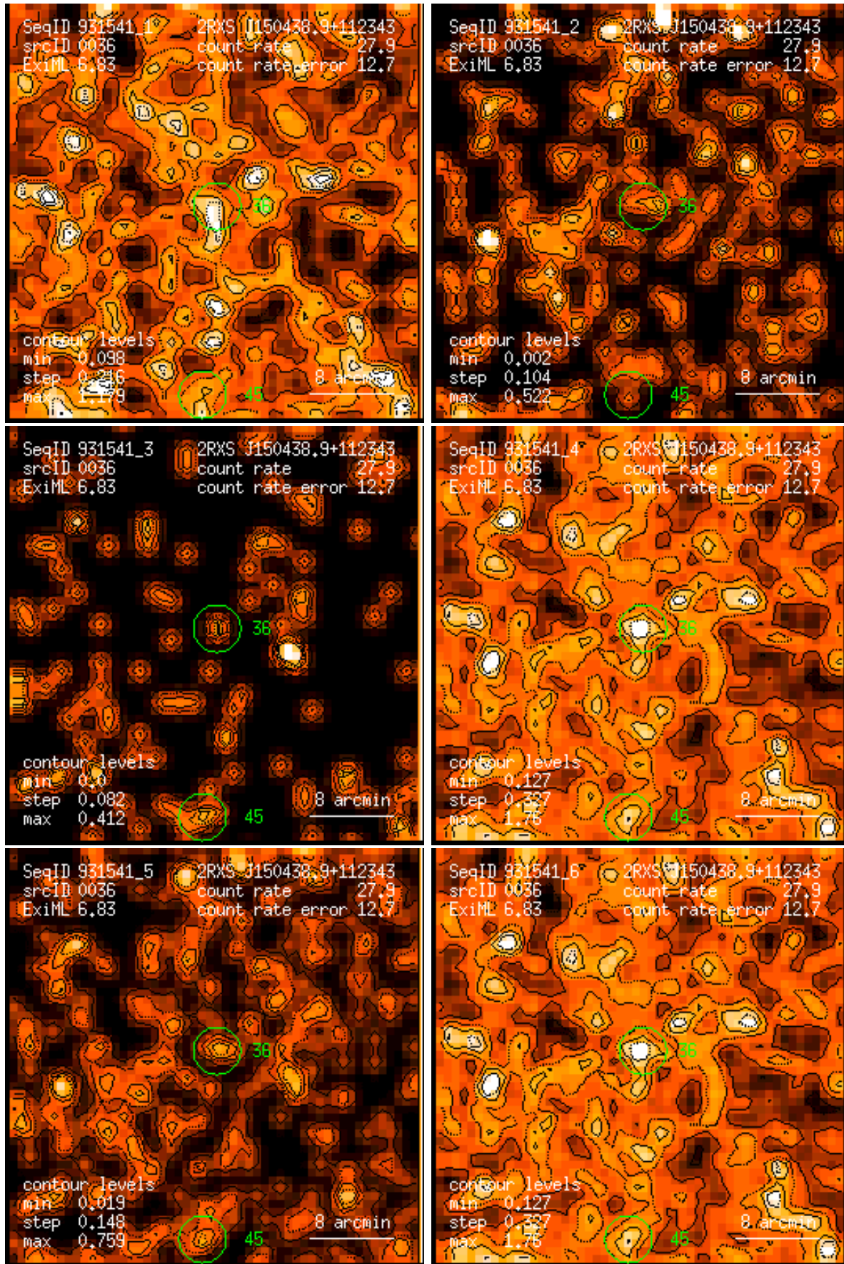
Figure 36: RASS 931541: detection 0036: band rate images, Gaussian filter: (1) PSPC channels 11 – 41, (2) 52 – 90, (3) 91 – 201, (4) 11 – 235, (5) 52 – 201, (6) 11 – 201. Broad band rates in counts/ks. Band rate contour levels in counts/ks/arcmin 2 .
